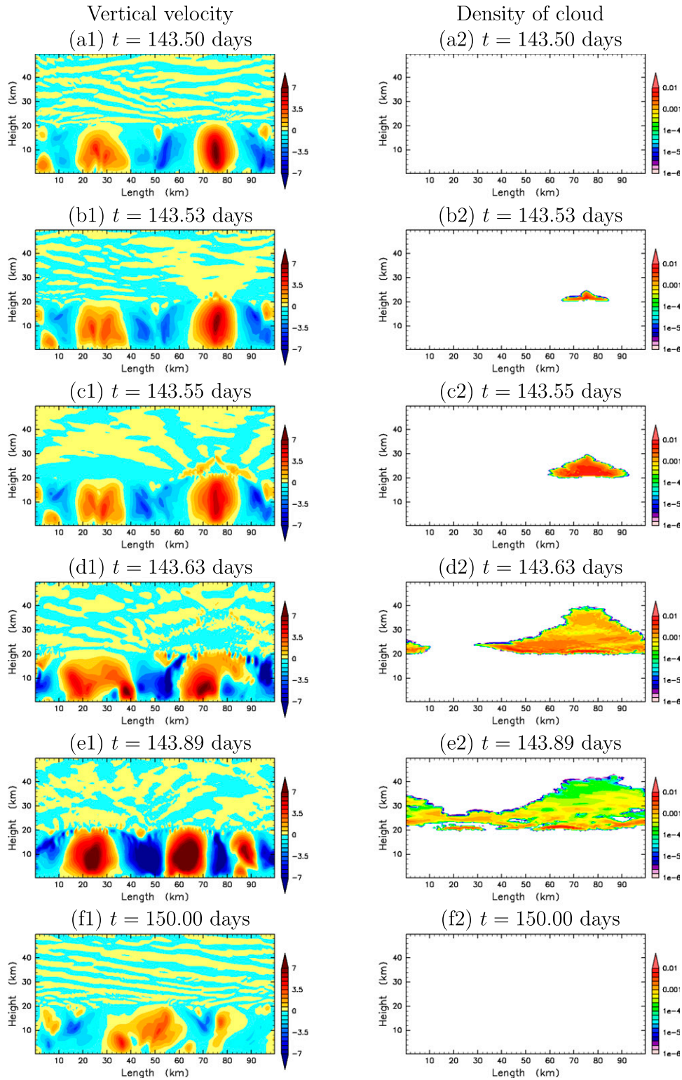
FIG. 5. Spatial distributions of (a1)–(f1) vertical velocity ( \text{m s}^{-1} ) and (a2)–(f2) mass density of \text{CO}_2 ice cloud ( \text{kg m}^{-3} ) for the case with S_{\text{cr}} = 1.35 and N_* = 5.0 \times 10^6 \text{ kg}^{-1} at (top to bottom) t = 143.50, 143.53, 143.55, 143.63, 143.89, and 150.00 days, respectively. Note that the time of (a) is equal to that of Figs. 6a,b and that of (c) is equal to that of Figs. 6c,d.
