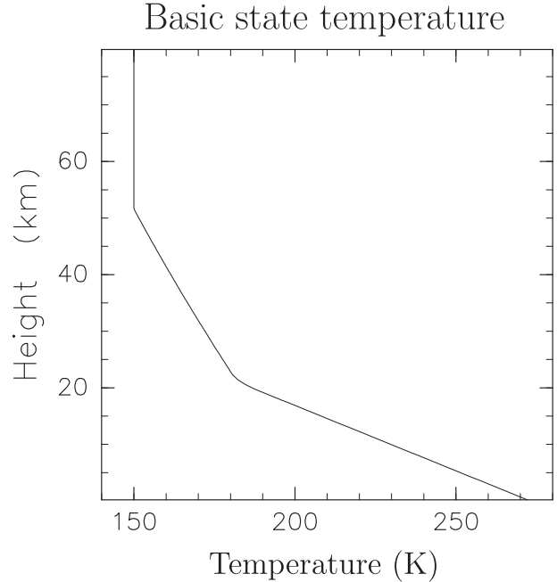
FIG. 1. Temperature profile of the basic state.
