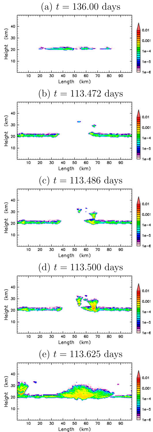
FIG. 11. Spatial distributions of mass density ( \text{kg m}^{-3} ) of \text{CO}_2 ice cloud for the case with (a) S_{cr} = 1.35 and N_* = 5.0 \times 10^4 \text{ kg}^{-1} during the period with clouds restricted around the condensation level ( t = 136.00 days) and with (b)–(e) those developing in higher altitudes ( t \sim 113.5 days).
