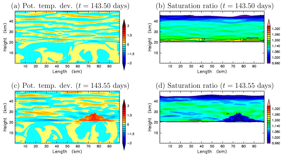
FIG. 6. Spatial distributions of (a),(c) potential temperature deviation from the horizontal mean (K) and (b), (d) saturation ratio in the case with S_{cr} = 1.35 and N_* = 5.0 \times 10^6 \text{ kg}^{-1} at (a),(b) t = 143.50 days, near the end of the noncondensation period, and (c),(d) t = 143.55 days in the early stage of the condensation period.
