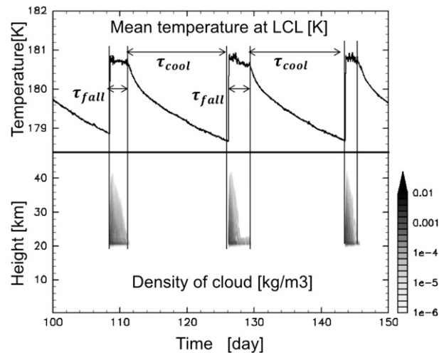
FIG. 7. (top) Time evolution of the horizontal-mean temperature (K) near condensation level ( z = 22.2 \text{ km} ) and (bottom) the vertical distribution of the horizontal-mean mass density ( \text{kg m}^{-3} ) of \text{CO}_2 ice cloud from t = 100 to 150 days in the case with S_{cr} = 1.35 and N_* = 5.0 \times 10^6 \text{ kg}^{-1} . The quantities \tau_{fall} and \tau_{cool} are the time scales of gravitational settling and radiative cooling, respectively (see text).
