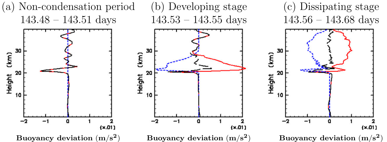
FIG. 8. Vertical profiles of the deviations of the accelerations due to thermal buoyancy (solid red line), due to drag force (dashed blue line), and due to net buoyancy (black line) from the corresponding horizontal means ( \text{m s}^{-2} ) for the case with S_{\text{cr}} = 1.35 and N_* = 5.0 \times 10^6 \text{ kg}^{-1} . (a) Last stage of noncondensation period averaged from t = 143.48 to 143.51 days, (b) early stage of condensation period averaged from t = 143.53 to 143.55 days, and (c) later stage of condensation period averaged from t = 143.56 to 143.68 days. Plotted are values averaged in an ascent region between x = 70 and x = 80 km.
