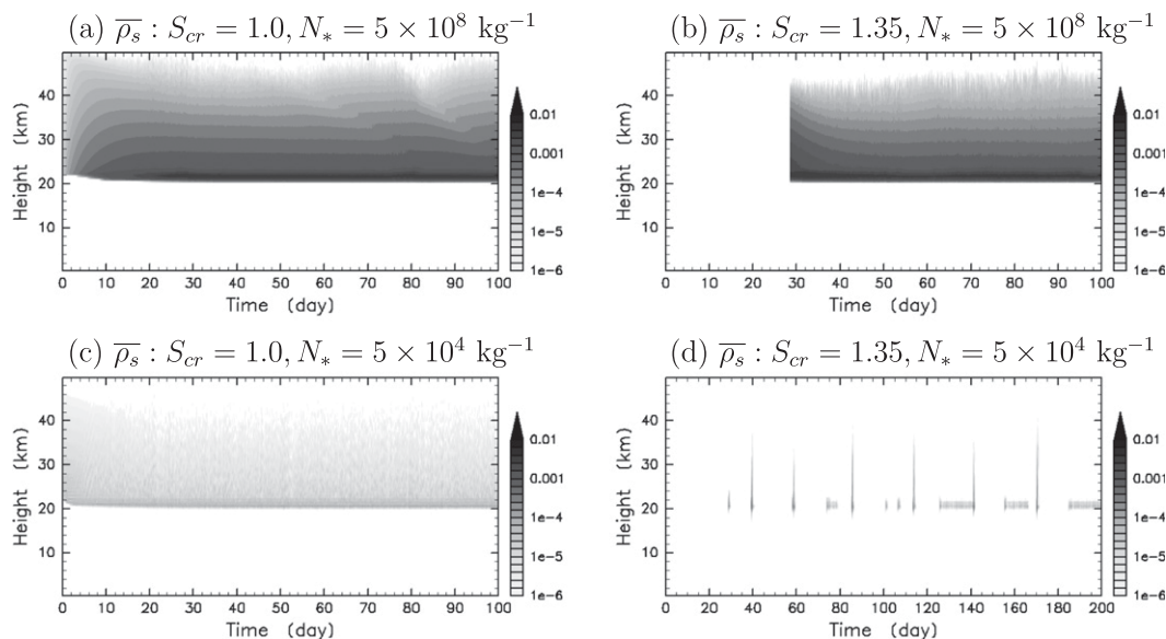
FIG. 9. As in Figs. 2c,d, but with (a),(b) N_* = 5.0 \times 10^8 and (c),(d) N_* = 5.0 \times 10^4 \text{ kg}^{-1} .
