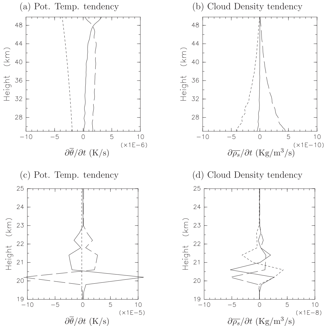
FIG. 12. Horizontal-mean tendencies of (a),(c) potential temperature (K) and (b),(d) cloud mass density ( \text{kg m}^{-3} \text{s}^{-1} ) averaged over the period between t = 90 and t = 100 days in the case with S_{\text{cr}} = 1.0 and N_* = 5.0 \times 10^6 \text{ kg}^{-1} . The altitudinal region from 25 to 50 km is shown in (a),(b) and that from 19 to 25 km in (c),(d). In (a),(c), plotted are the sum of the advection term and the turbulent diffusion term (solid line), the condensation heating term (line with long dashes), and the radiative cooling term (line with short dashes). In (b),(d), plotted are the sum of the advection term and the turbulent diffusion term (solid line), the condensation term (line with long dashes), and the gravitational settling term (line with short dashes).
