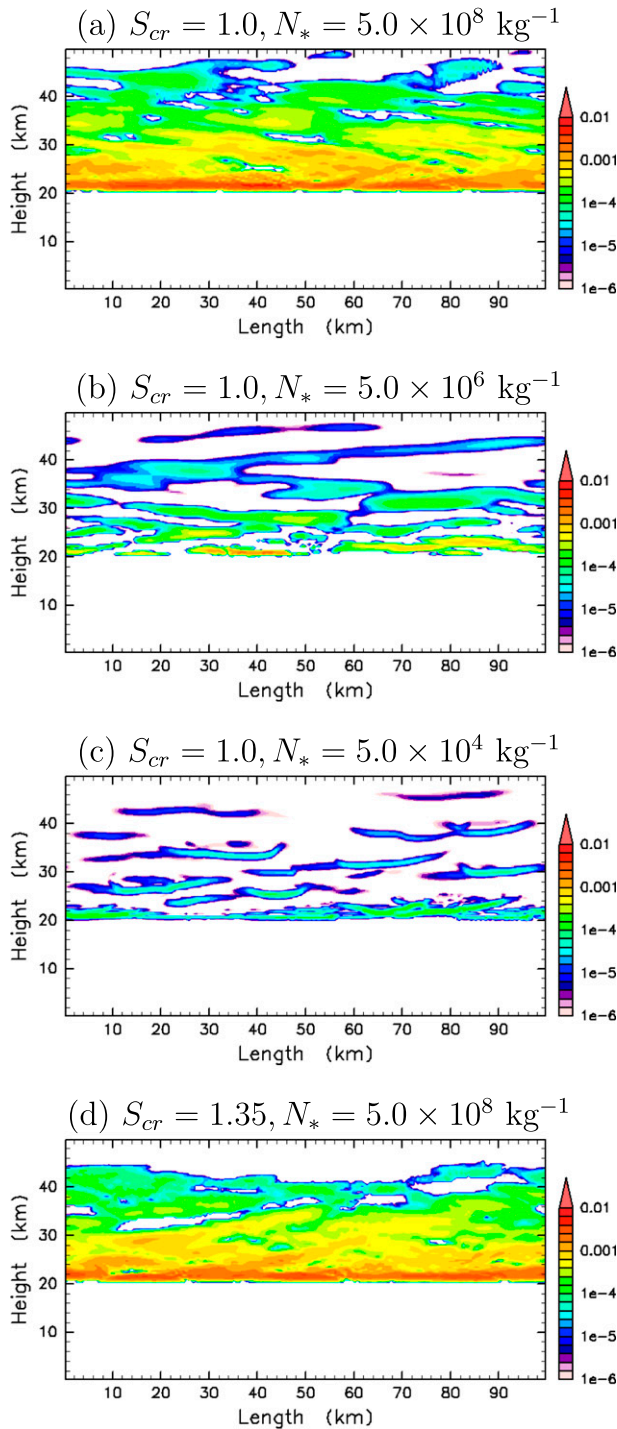
FIG. 10. Spatial distributions of mass density ( \text{kg m}^{-3} ) of \text{CO}_2 ice cloud at t = 100 days in the cases with S_{cr} = 1.0 and (a) N_* = 5.0 \times 10^8 , (b) N_* = 5.0 \times 10^6 , and (c) N_* = 5.0 \times 10^4 \text{ kg}^{-1} , and with (d) S_{cr} = 1.35 and N_* = 5.0 \times 10^8 \text{ kg}^{-1} .
