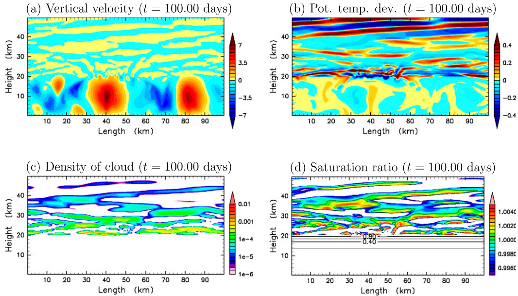
FIG. 3. Spatial distributions of variables at t = 100 days for the case with S_{\text{cr}} = 1.0 and N_* = 5.0 \times 10^6 \text{ kg}^{-1} . (a) Vertical velocity ( \text{m s}^{-1} ), (b) potential temperature deviation from the horizontal mean (K), (c) mass density of \text{CO}_2 ice cloud ( \text{kg m}^{-3} ), and (d) saturation ratio.
