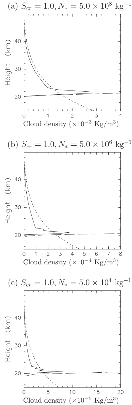
FIG. 13. Time- and horizontal-mean mass density of CO 2 ice cloud obtained by simulation (solid line), mass density of CO 2 ice cloud obtained under the assumption of constant CO 2 ice static energy (line with long dashes), and that obtained under the assumption of the balance of condensation and gravitational settling and the balance of condensation heating and horizontally uniform cooling (line with short dashes) for the cases with (a) N_* = 5.0 \times 10^8 , (b) N_* = 5.0 \times 10^6 , and (c) N_* = 5.0 \times 10^4 \text{ kg}^{-1} . All cases shown here are of S_{cr} = 1.0 , and simulation data are averaged over the period between t = 110 and t = 120 days.
