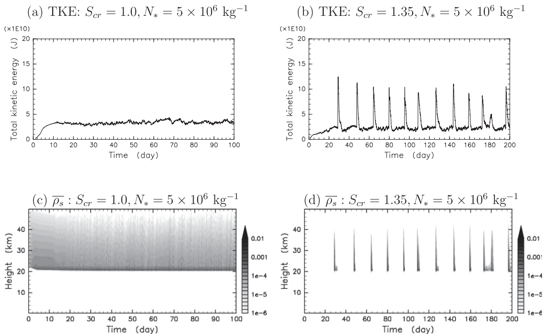
FIG. 2. Temporal evolutions of (a),(b) total kinetic energy ( \text{J} \times 10^{10} ) and (c),(d) horizontal-mean cloud density ( \text{kg m}^{-3} ) for the two runs using two different values of S_{cr} with N_* = 5.0 \times 10^6 \text{ kg}^{-1} . (a),(c) The evolutions from 0 to 100 days are shown for the case with S_{cr} = 1.0 and (b),(d) the evolutions from 0 to 200 days are shown for the case with S_{cr} = 1.35 . In (c) and (d), a logarithmic gray scaling is used with minimum value of shading set as \rho_s = \rho_s^7 = 10^{-6} \text{ kg m}^{-3} .
