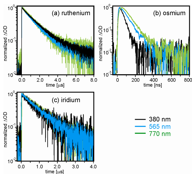
Figure 5. Decays of the transient absorption intensities from Figure 4 at three different wavelengths in the TAA-Ru II -AQ (a), TAA-Os II -AQ (b), and TAA-Ir III -AQ (c) triads in de-oxygenated CH 3 CN solution at 25°C. Excitation occurred at 532 nm for the ruthenium and osmium triads and at 355 nm for the iridium system.
