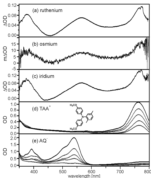
Figure 4. Panels (a) – (c) show transient absorption spectra measured on \text{CH}_3\text{CN} solutions of TAA- \text{Ru}^{\text{II}} -AQ (a), TAA- \text{Os}^{\text{II}} -AQ (b), and TAA- \text{Ir}^{\text{III}} -AQ (c) in a 200-ns time window starting immediately after excitation with \sim 10 -ns laser pulses at 532 nm (a, b) or 355 nm (c). Panel (d) shows a series of absorption spectra from a \text{CH}_2\text{Cl}_2 solution of a triarylamine reference molecule (structure shown in the inset) after increasing time intervals following application of an electrochemical potential more positive than 0.5 V vs. \text{Fc}^+/\text{Fc} (in presence of 0.1 M \text{TBAPF}_6 ). Panel (e) shows a series of absorption spectra obtained from a \text{CH}_2\text{Cl}_2 solution of 9,10-anthraquinone obtained in an analogous spectro-electrochemical experiment using potentials more negative than -1.2 V vs. \text{Fc}^+/\text{Fc} .
