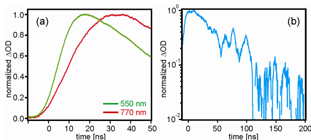
Figure 7. (a) Rise of the transient absorption signals at 550 nm (green trace) and 770 nm (red trace) after excitation of the TAA-Os II -AQ triad at 532 nm with laser pulses of ~10 ns width (CH 3 CN solution). (b) Decay of the transient absorption signal of the Os II -AQ dyad at 550 nm (AQ - disappearance) after excitation at 532 nm with laser pulses of ~10 ns width (de-oxygenated CH 3 CN solution).
