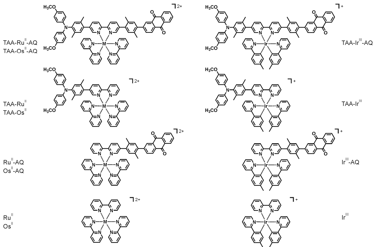
Scheme 2. The molecules investigated in this work. TAA = triarylamine; AQ = anthraquinone.
