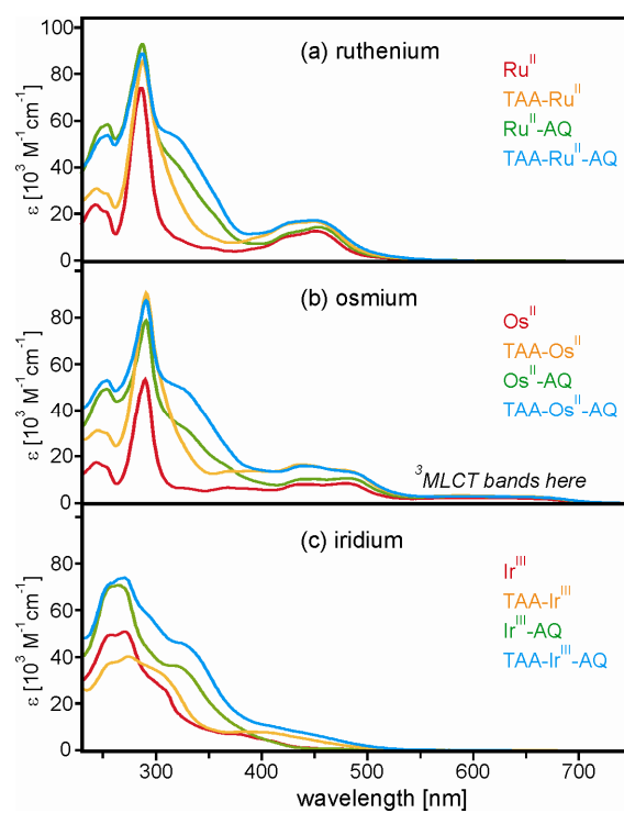
Figure 1. Optical absorption spectra of the 12 molecules from Scheme 2 in CH 3 CN at 25°C.
