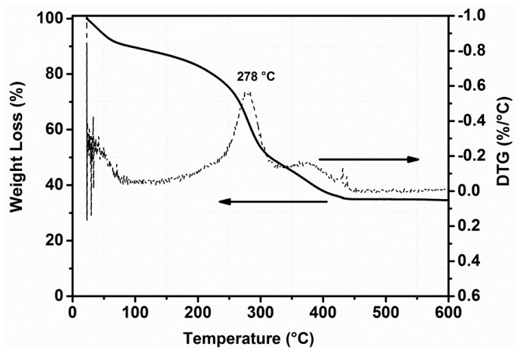
Figure S1-TGA/DTG profile for the V-W-TiO 2 nanofibers.
