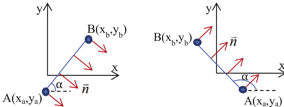
Fig. 3. Definition of flux through straight segments. Left: Positive direction of flux for 0 \leq \alpha \leq \frac{\pi}{2} . Right: Positive direction of flux for \frac{\pi}{2} < \alpha < \pi .
