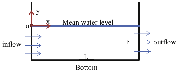
Fig. 17. Sketch of numerical wave tank.
