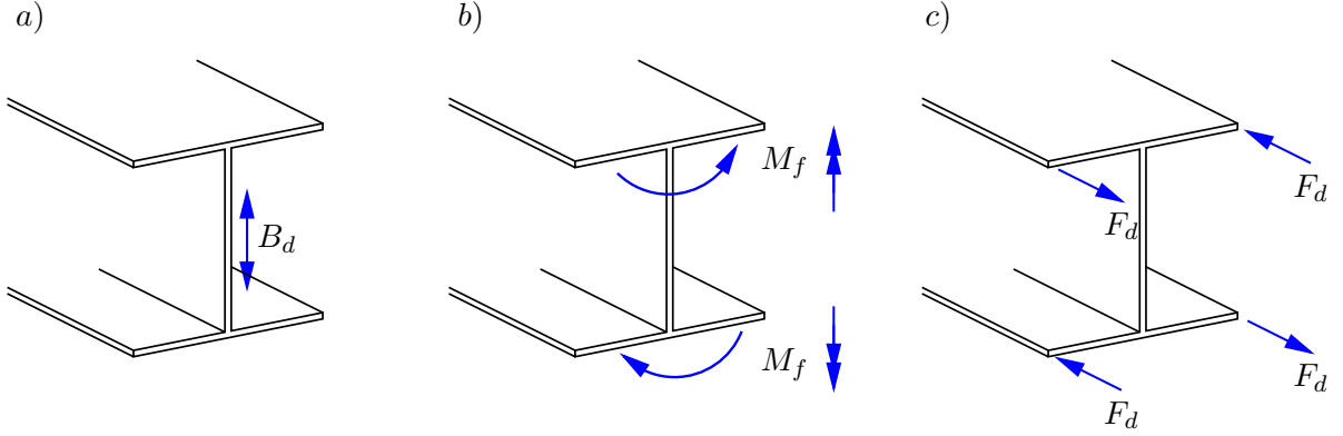
Figure 2: I-profile beam with a bimoment a) , bending moments at the flanges generating the bimoment b) and equivalent configuration of concentrated, axial forces c) .
