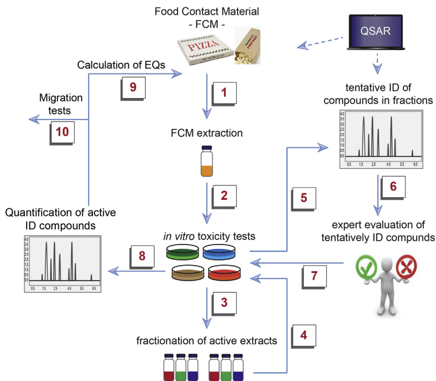
Fig. 1. Workflow for the effect-directed strategy for FCMs made from paper and board, 1) preparation of FCM extracts from paper and board, 2) in vitro testing of extracts, 3) fractionation of active extracts, 4) in vitro testing of fractions, 5) tentative compound identification in active fractions, 6) selection of final list of test compounds, 7) in vitro testing of final list compounds, 8) identification and quantification of compounds, 9) calculation of equivalence factors (EQs), 10) migration studies. ID = identification.
