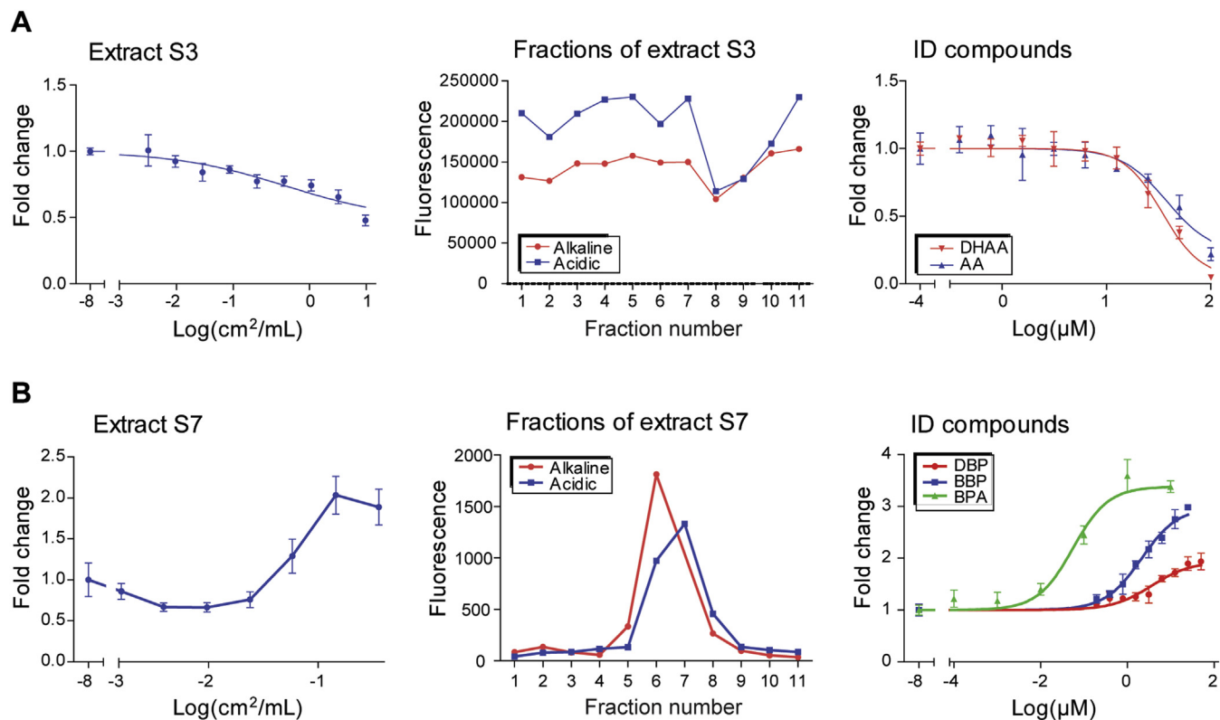
Fig. 3. In vitro data from workflow described in Fig. 1. Biological activity of FCM extracts (left), fractions of extracts (middle), and identified (ID) biologically active compounds in active fractions and extracts (right). A) Androgen receptor (AR) antagonism of sandwich wrapper (S3) extract and fractions as well as compounds therein. B) Estrogen receptor (ER) agonism of the pizza box (S7) extract and fractions as well as compounds therein. Graphs are based on one representative experiment of extract, fractions, and ID compounds (means \pm SD). BPA data has previously been published in Rosenmai et al., (2014).
