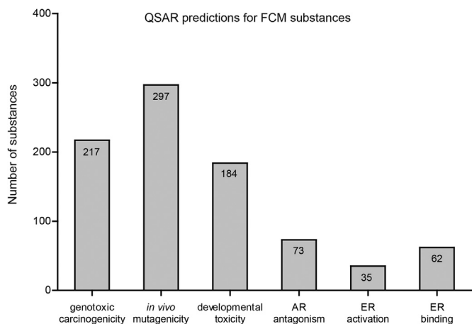
Fig. 2. QSAR predictions for genotoxic carcinogenicity, in vivo mutagenicity, developmental toxicity, in vitro estrogen receptor (ER) activation and binding, and androgen receptor (AR) antagonism for 2076 FCM compounds.
