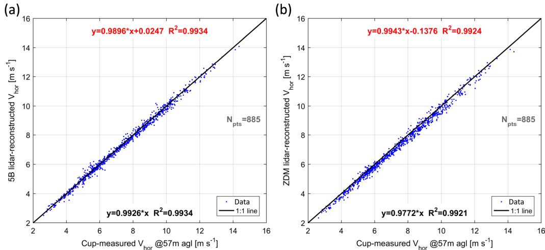
Figure 10. Comparison between mast-measured and lidar-estimated horizontal wind speed at 57.5 m height a.g.l and 2.5D_{rot} using short-range measurements. (a) 5B-Demo lidar, using five LOS and four ranges. (b) ZDM lidar, using six LOS and three ranges.
