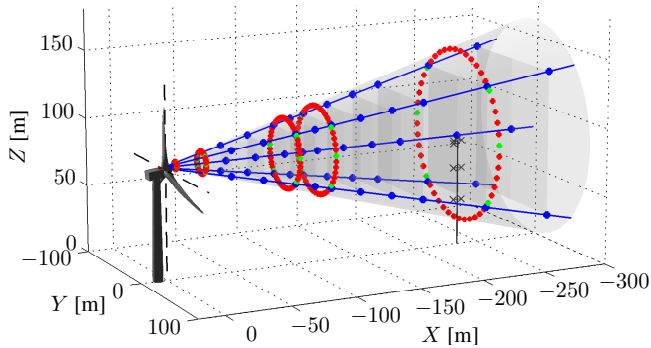
Figure 5. Lidar measurement trajectories in NKE. In blue: five-beam Avent Demonstrator. In red and green: ZephIR Dual Mode, the 48 azimuth-averaged LOS (red), including the 6 LOS (green) considered in the reconstruction cases of this paper.
