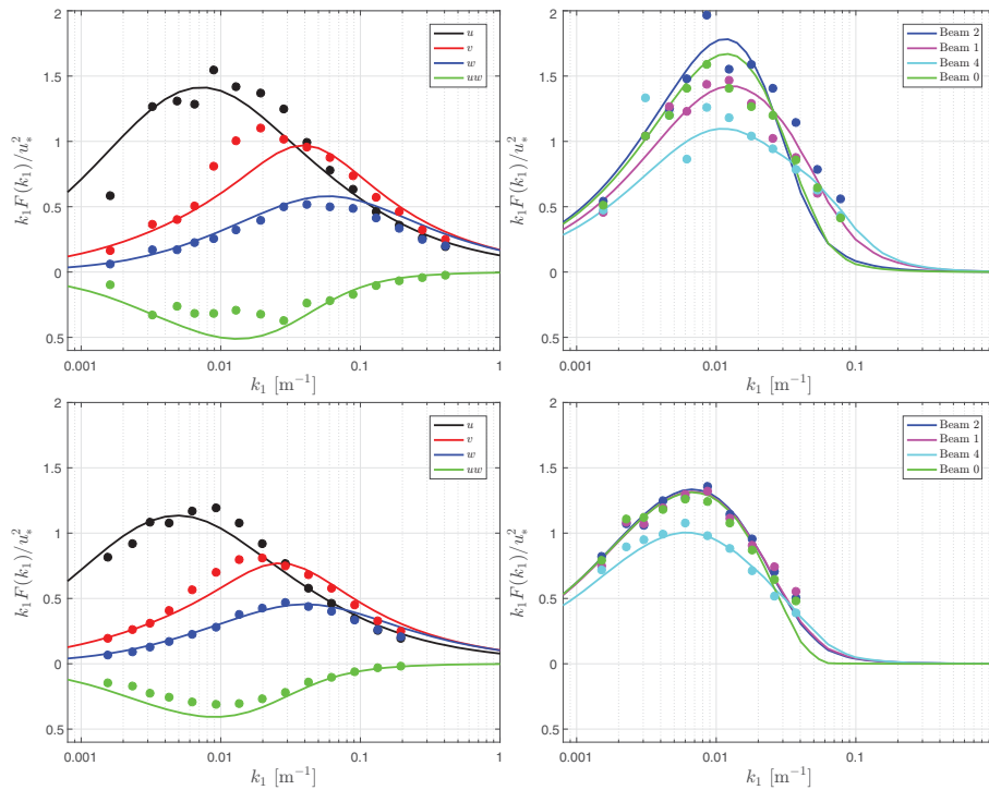
Figure 19. Similar to Fig. 17, but here the top panels show the results for the first wind-speed range (speed 1) and the bottom panels for the last wind-speed range (speed 5).
