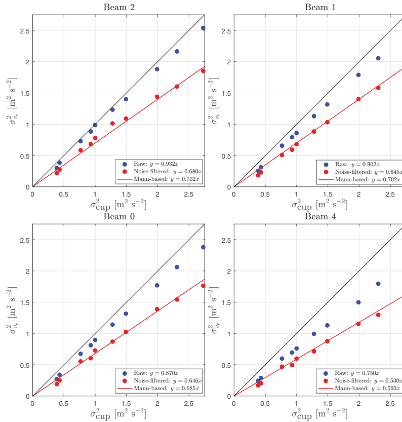
Figure 16. Comparison of the 80 m cup anemometer with the Avert radial velocity variances for different beams for the 10 turbulence classes (filled circles) in Table 1. Raw and noise-filtered data are shown as well as a 1 : 1 line (for guidance) and the prediction of the Avert filtered radial velocity variance based on the Mann model, using \Gamma = 3.00 , L = 35.38 m, and \beta = 0^\circ .
