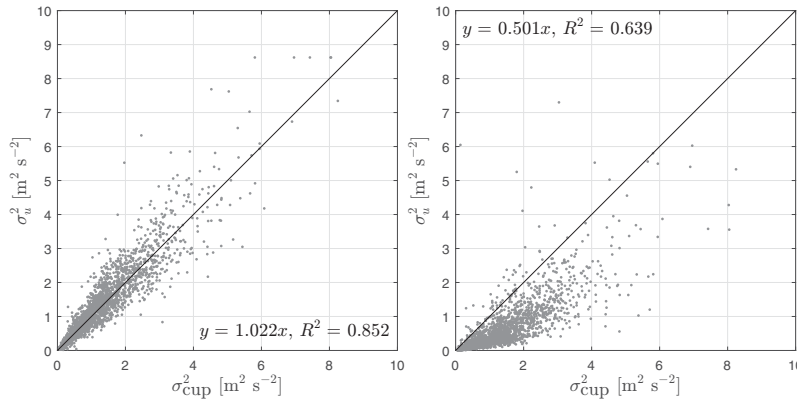
Figure 15. Comparison of the 80 m cup anemometer and the unfiltered (left) and filtered (right) u variances from the ZephIR estimated under the assumption of homogeneous turbulence within the measurement volume (see text for details). We show a 1 : 1 line for guidance. Results of a linear regression through the origin and R^2 are also given.
