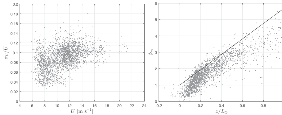
Figure 13. (Left) Turbulence intensity \sigma_U/U as a function of mean wind speed U from the 80 m cup-anemometer observations. (Right) Dimensionless wind shear \phi_m as a function of dimensionless stability, z/L_0 , based on the sonic- and cup-anemometer observations. The grey markers show 2273 10 min concurrent samples and the solid lines are theoretical predictions (see text for details).
