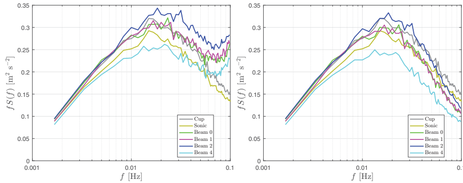
Figure 10. Ensemble-average spectrum of all 10 min Avent radial velocity spectra (per beam), sonic-anemometer u spectrum, and 80 m cup-anemometer spectrum. Original (left) and noise-filtered lidar radial velocity spectra (right).
