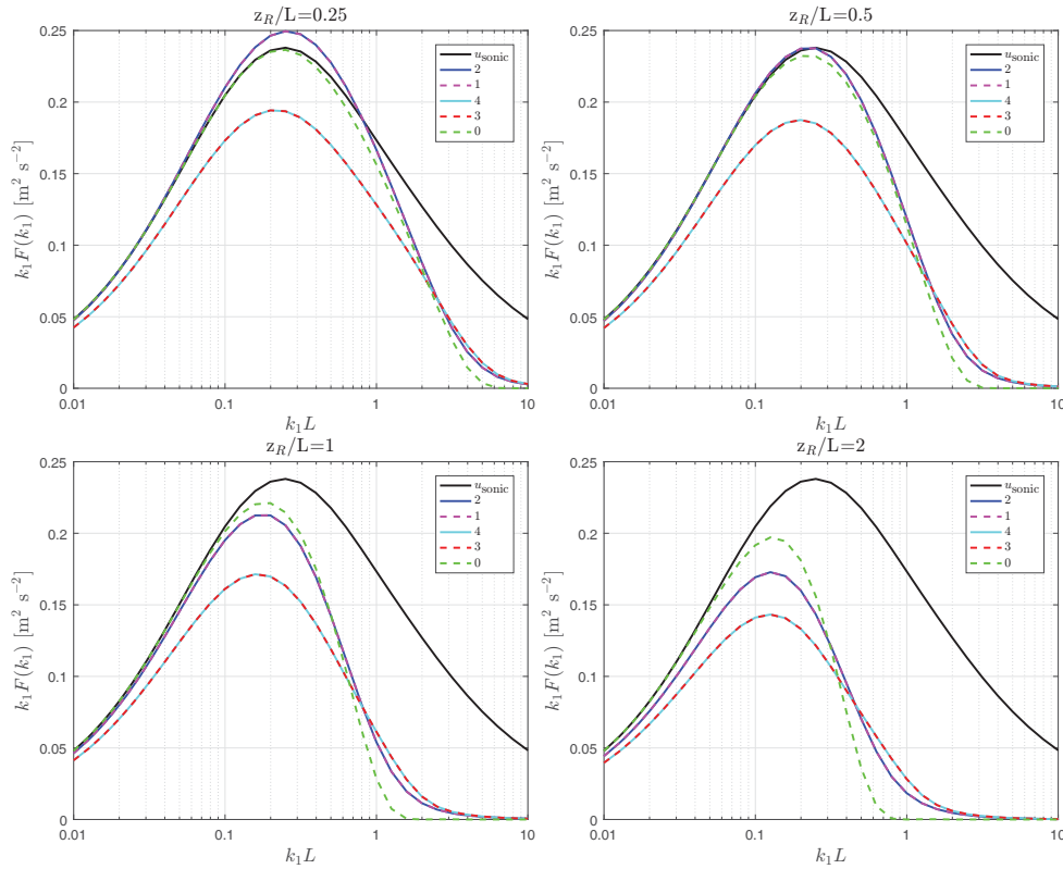
Figure 3. Sonic and pulsed lidar velocity spectra from Eqs. (3) and (6) corresponding to the beams shown in Fig. 1 (right panel). Values of z_R/L are indicated, \varphi = 15^\circ , \Gamma = 3 , and \alpha \varepsilon^{2/3} = 0.1 \text{ m}^{4/3} \text{ s}^{-2} .
