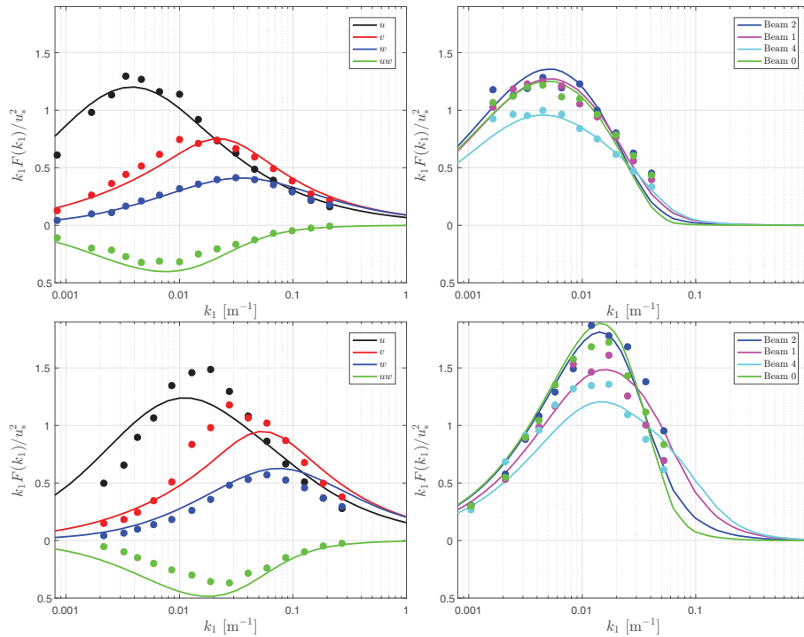
Figure 17. Normalized power spectra of the different velocity components based on the sonic-anemometer observations (left) and of the Avent radial velocity for different beams (right). The top panels show the results for the first stability range (stability 1) and the bottom panels for the last stability range (stability 5).
