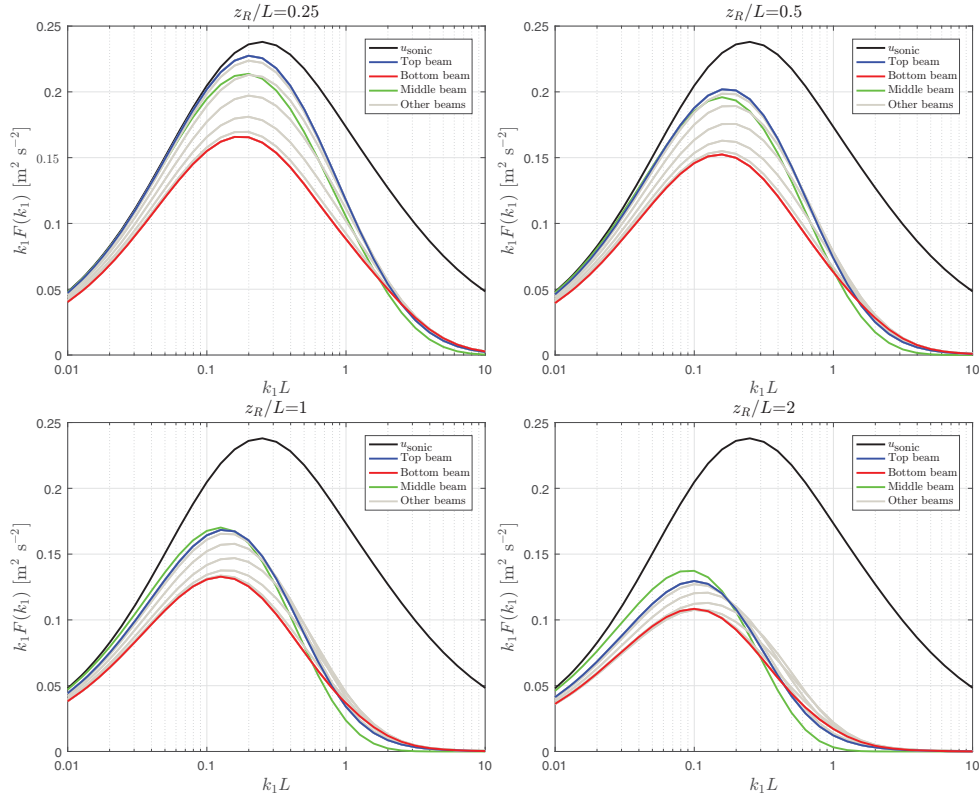
Figure 2. Sonic and CW lidar velocity spectra from Eqs. (3) and (6), corresponding to the beams shown in Fig. 1 (left panel). Values of z_R/L are indicated, \varphi = 15^\circ , \Gamma = 3 , and \alpha\varepsilon^{2/3} = 0.1 \text{ m}^{4/3} \text{ s}^{-2} .
