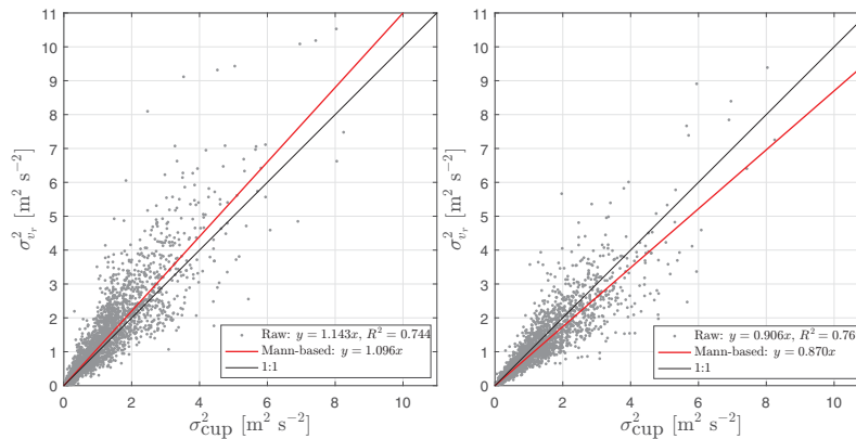
Figure 14. Comparison of the 80 m cup-anemometer and the unfiltered ZephIR radial velocity variances for bins 0 (left) and 31 (right). We show a 1 : 1 line for guidance and the predictions of the Mann model using \Gamma = 3 . Results of a linear regression through the origin and R^2 are also given. For bin 31, \sigma_{v_r}^2 > 11 m 2 s -2 for two 10 min periods.
