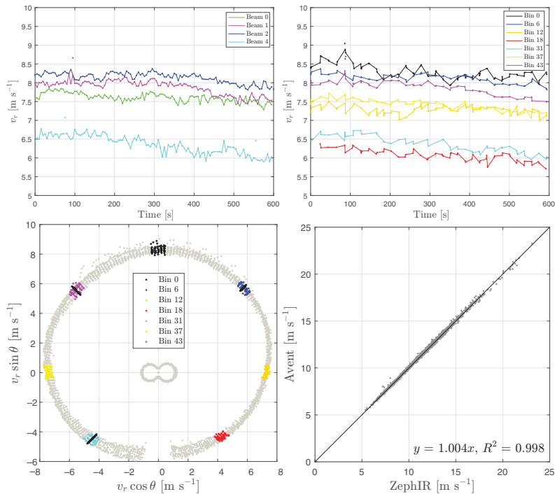
Figure 7. An example of a 10 min time series of the radial velocity of different beams for the Avent (top left) and the ZephIR (top right) lidar. The radial velocities of the two lidars at all azimuthal positions are illustrated in the bottom-left panel (see text for details). In the bottom-right panel, we show a comparison of the 2273 10 min mean radial velocities of the Avent (beam 2) and ZephIR (bin 6) with the results of a linear regression through the origin and coefficient of determination R^2 . Measurements from beam 3 of the Avent are omitted due to low availability.
