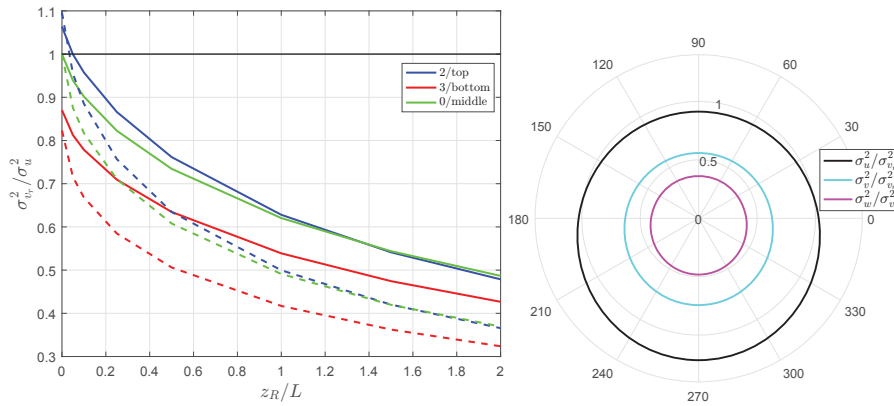
Figure 4. (Left) Variance of the lidar beams’ radial velocity (divided by the u component variance) of the 2/top, 3/bottom and 0/middle beams of the pulsed/CW (solid/dashed lines) lidars as a function of z_R/L . (Right) Ratio of the variance of each of the velocity components to that of lidar beam as function of azimuthal position for z_R/L = 0 . Turbulence characteristics are computed for \varphi = 15^\circ and \Gamma = 3 .
