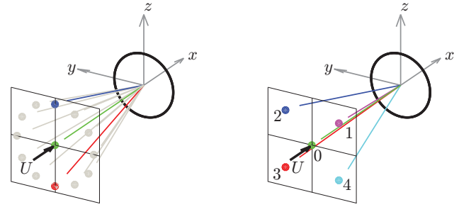
Figure 1. Geometry of the rotor and nacelle lidars. The x axis is in the mean wind direction. The lidar beams point upwind in the directions determined by the unit vectors \mathbf{n}_i . For the CW lidar (left frame) we include a beam perpendicular to the rotor for comparison only. For the pulsed lidar (right frame) we show a five-beam configuration where beam 0 is perpendicular to the rotor. Beams perpendicular to the rotor are shown in green (beam 0), top beams in blue and magenta (beams 1 and 2), bottom beams in red and cyan (beams 3 and 4), and other beams in grey.
