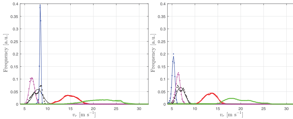
Figure 12. Examples of normalized Doppler radial velocity spectra measured over five 10 min periods with the ZephIR at the positions of bin 0 (left) and bin 31 (right). The markers show the observed distributions and the solid lines show a normal fit.
