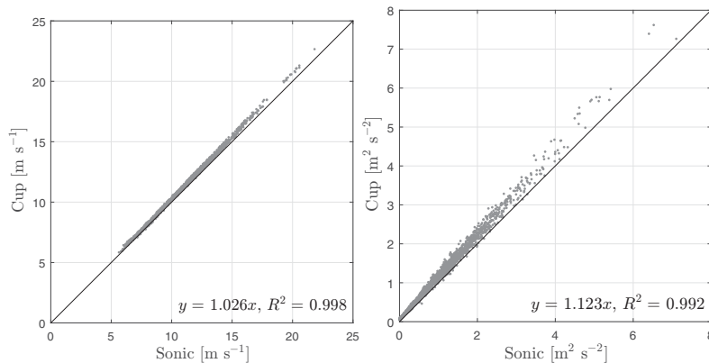
Figure 8. Comparison of sonic and 80 m cup anemometer statistics: mean wind speed (left frame) and horizontal-wind variance (right frame). Each 10 min sample is shown in grey markers, a 1 : 1 line is shown for guidance in black, and the results of a linear regression through the origin and R^2 are given.
