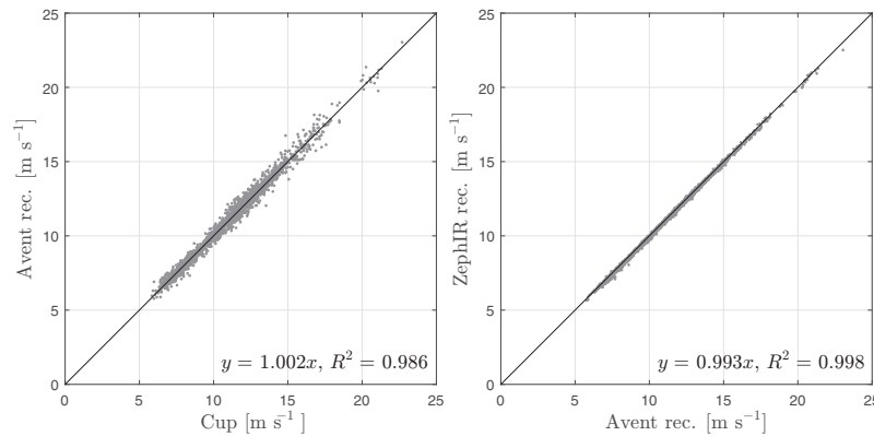
Figure 11. Comparison of reconstructed and 80 m cup anemometer horizontal wind speeds. (Left) Cup anemometer against Avent. (Right) Avent against ZephIR. Each 10 min sample is shown in grey markers. A 1 : 1 line is shown for guidance in black, and the results of a linear regression through the origin and R^2 are also given.
