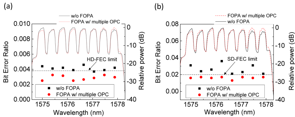
Fig. 8. Spectra (right axis) and BERs (left axis) after 3600 km transmission and 6000 km transmission of 8 channels for the cases of 'w/o FOPA' and 'FOPA w/ multiple OPC'.
