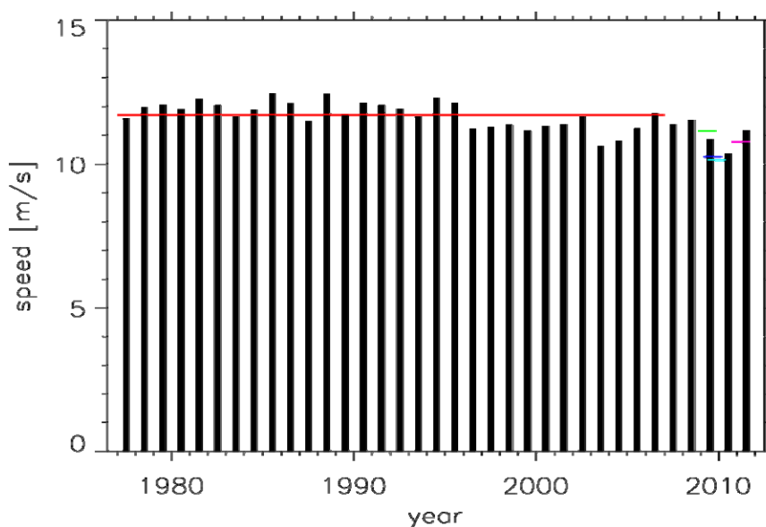
Figure 3. Variation of the annual large scale mean geostrophic wind speed from year to year (vertical bars) for Mali with indication of the thirty-year average value (red line) and the mean value for the different measurement periods (green, purple, blue and pink lines).
