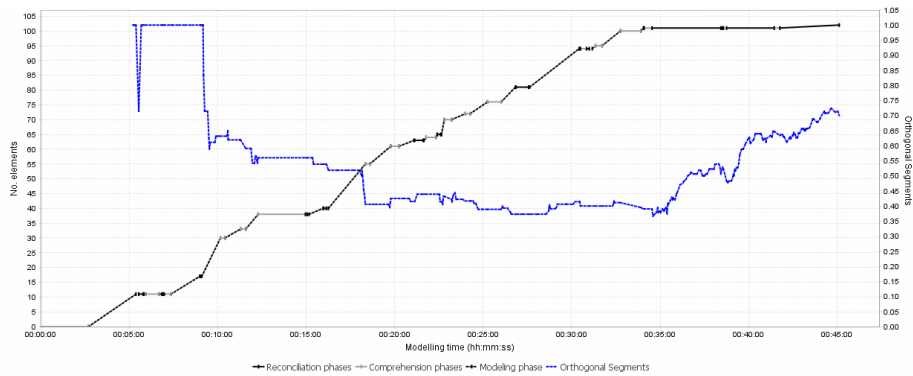
Fig. 2. An advanced modeling phase diagram with the orthogonal segments metric
