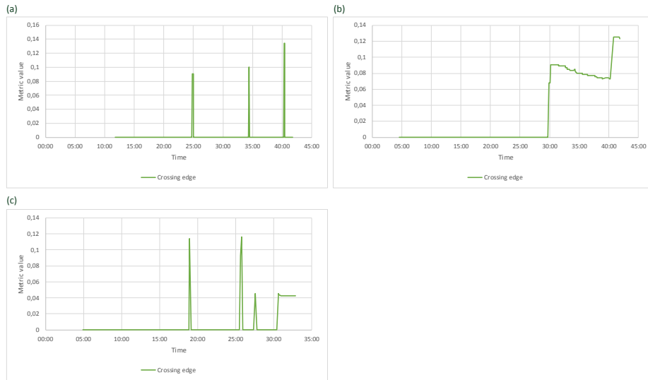
Fig. 3. Examples for the evolution of the crossing edge metric
