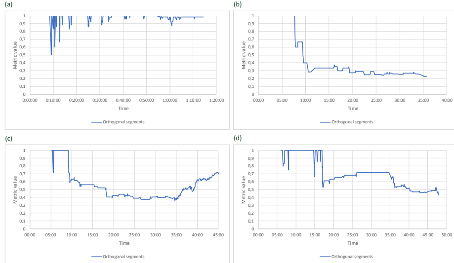
Fig. 4. Examples for the evolution of the orthogonal segments metric
