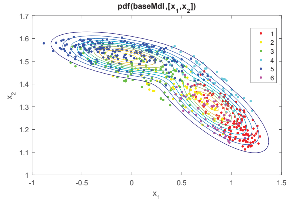
Fig. 6. Scatterplot of sum of log-cos-distance to undesirable shapes x_1 vs. sum of log-cos-distance to desirable shapes x_2 ; the data points are coloured by associated base shape clusters ( desirable BS : {1, 2, 4, 6}; undesirable BS : {3, 5}). The data is overlaid with the two-parameter GM to be used for response type identification: upper-left: undesirable response shape, lower-right: desirable response shape.
