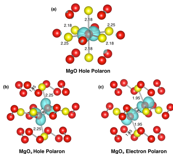
Figure 3. Magnetization density for (a) hole polaron in MgO, (b) hole polaron in MgO 2 , and (c) electron polaron in MgO 2 . The isosurface is plotted at 0.01 \text{ e}/\text{\AA}^3 . The numbers in the figure indicate bond length in Å. The oxygen to Mg bond distance in bulk is 2.1 Å for both MgO and MgO 2
