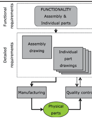
Figure 1 Connection between specification, manufacturing and quality assurance.
