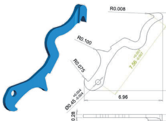
Figure 4 A ceramic knocker for high-end watch. Two critical dimensions with symmetric tolerances are noted in the drawing [11].
