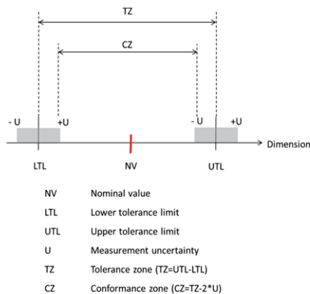
Figure 2 Symmetrical dimensional tolerance
