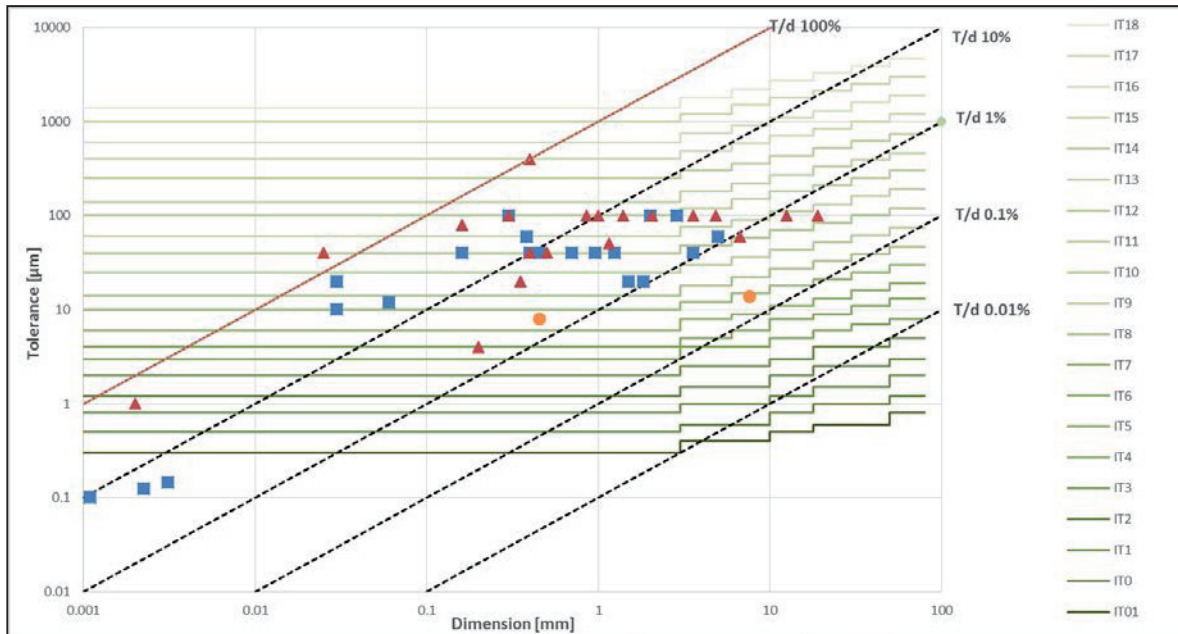
Figure 3 Tolerance vs. dimension. The blue square dots are for polymer parts, the red triangular dots are for metal parts; the orange circular dots are for ceramic components. The green lines show the tolerance values for different dimension ranges in the ISO 286 standard, while the different shades of green stand for different tolerance grades. The dashed lines are contour plots for Tolerance/ dimension ratio. [4], [8]-[18]
