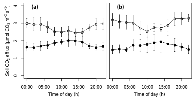
Figure 9. Diurnal pattern of soil CO 2 efflux measured by the automated chambers during the fan experiment, based on bi-hourly means ( \pm standard deviation). Panel (a) shows the diurnal pattern for half of the chambers with and without fans, where the first 10 days were with fans (filled circles) and the last 10 days were without fans (open circles). Panel (b) shows the diurnal pattern with and without fans for the other half of the chambers, where the first 10 days were without fans (open circles) and the last 10 days were with fans (filled circles).
