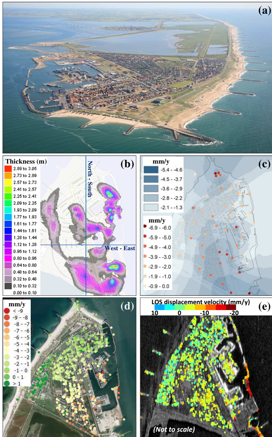
Figure 3. Thyboron: photo towards south (by courtesy of Hunderup Aerial Photography/Danish Coastal Authority)(a); isopach map of gyttja/soft sediments (b); measured and interpolated vertical rates of land movement (subsidence is negative) from precision leveling (2006-2015) (c); measured rates from ERS2 (1995-2001) satellite imagery (d), and measured 'line-of-sight' (LOS) rates from Sentinel-1(2015-2016) satellite imagery (e).
