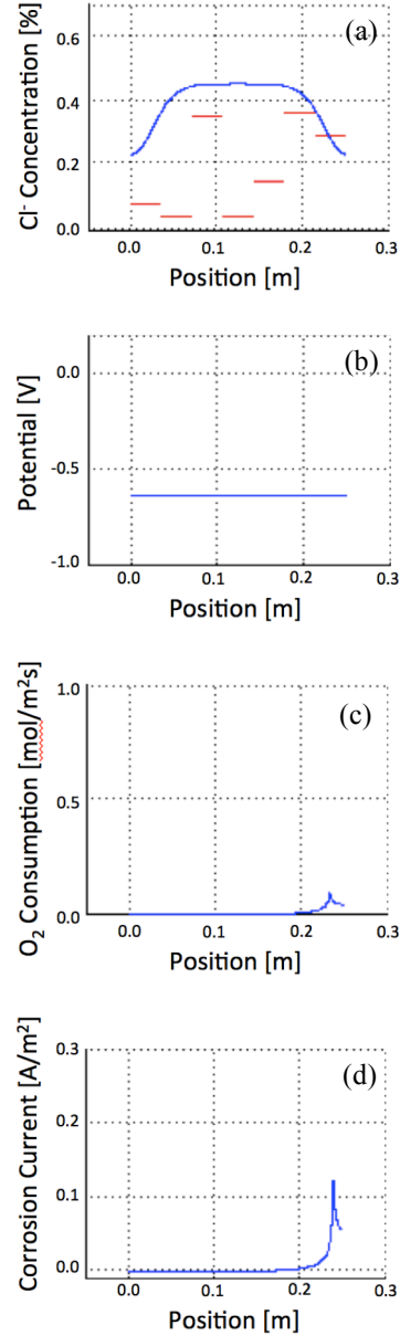
Figure 7: Distribution along the cracked reinforced HPRCC member of (a) \text{Cl}^- ion concentration at the rebar surface, (b) potential, (c) \text{O}_2 consumption, and (d) corrosion current at 200 months
