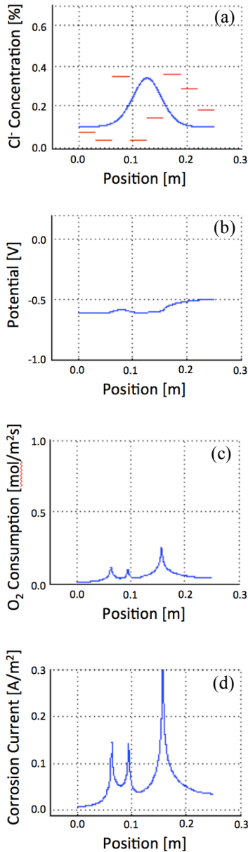
Figure 5: Distribution along the cracked reinforced concrete member of (a) Cl - ion concentration at the rebar surface, (b) potential, (c) O 2 consumption, and (d) corrosion current at 200 months
