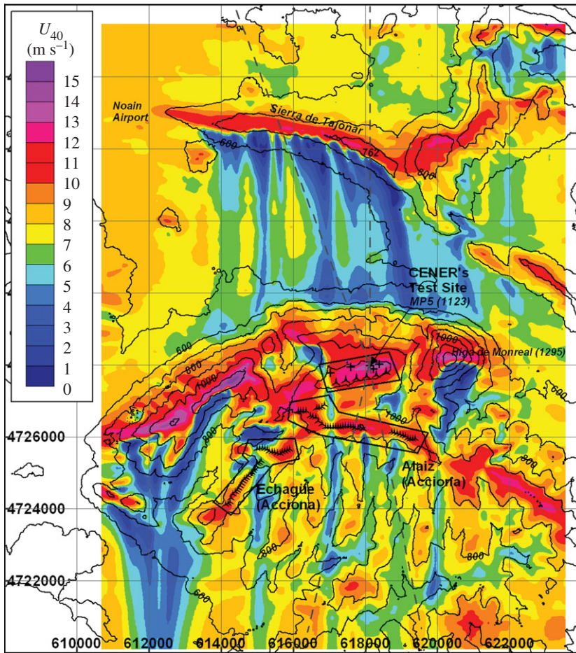
Figure 14. Contour map of horizontal wind speed at 40 m a.g.l. simulated with CFDWind [53]. Wind direction from the North. Northern and Southern sectors of interest for the Alaiiz experiment delimited by dashed lines and centred at the MP5 position of CENER's Test Site. (Online version in colour.)
