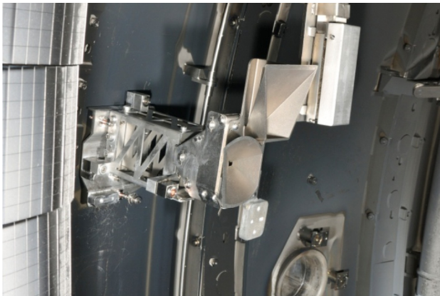
Fig. 4. ITER First Mirror installed in JET.
