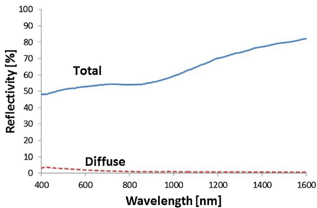
Fig. 3. Reflectivity of one of the mirror samples.
