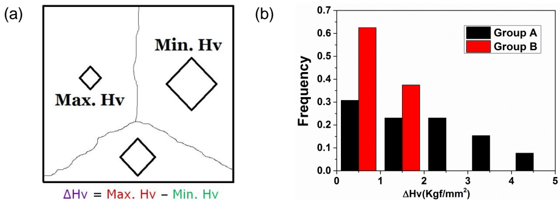
Figure 3.9: (a) Sketch showing the calculation of the microhardness difference at triple junctions. (b) The distribution of the microhardness difference between the maximum and minimum hardness at Group A and Group B triple junctions. (b) is reproduced from article A.
