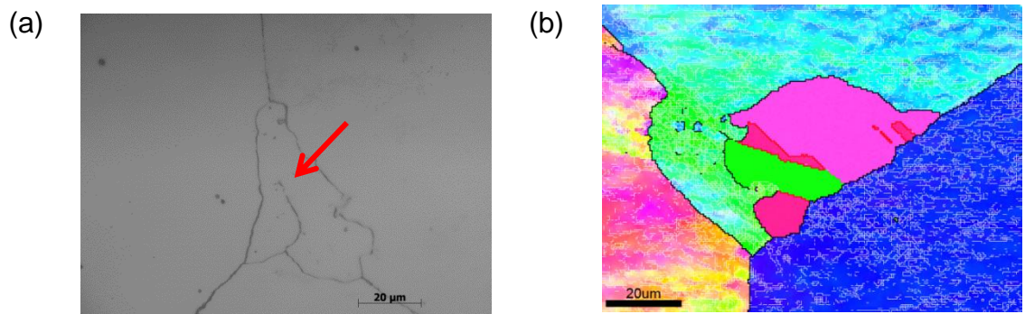
Figure 3.4: (a) Optical micrograph of a nucleus (marked by an arrow) formed at a triple junction and (b) orientation map of nuclei formed at grain boundaries
