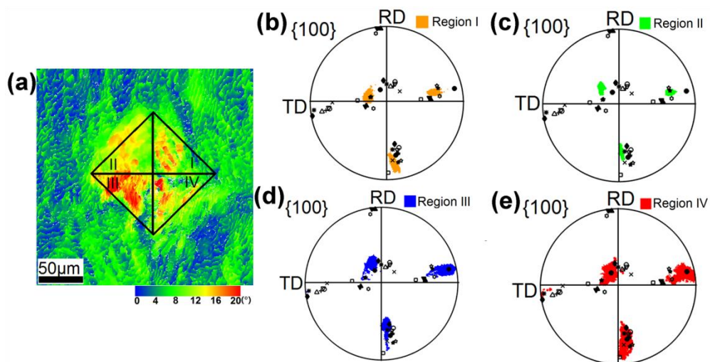
Figure 4.23: (a) EBSD map showing the regions of I, II, III and IV, and (b)-(e) \{100\} pole figures of all the 1-h and 2-min nuclei within the 4 regions: I - IV, in (a). Reproduced from article C.
