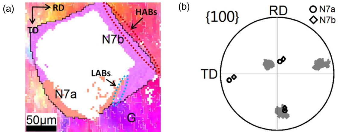
Figure 4.12: (a) EBSD orientation map and (b) \{100\} pole figure of the recovered matrix and the nuclei N7a and N7b formed at Grain E. The grey 'cloud' in the pole figure represents the orientations within the recovered matrix G and the circles and the diamonds show the orientations of the nuclei N7a and N7b, respectively. The color code in (a) is same as that in figure 4.11(a).
