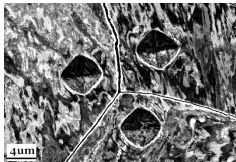
Figure 3.7: Example showing the microhardness tests around a triple junction. Reproduced from article A.
