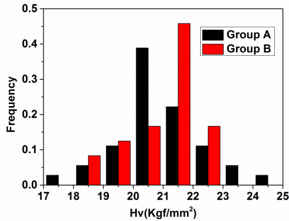
Figure 3.8: Distribution of microhardness of all 3 grains at Group A and Group B triple junctions. Reproduced from article A.
