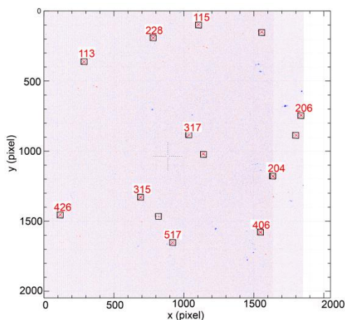
Figure 5.1: An example of a depth-resolved Laue diffraction pattern from a voxel within the deformed volume 75\ \mu\text{m} below the sample surface. The indexed diffraction spots are marked by squares and the hkl indexes of the identified diffracting crystallographic planes are given. Reproduced from article D.
