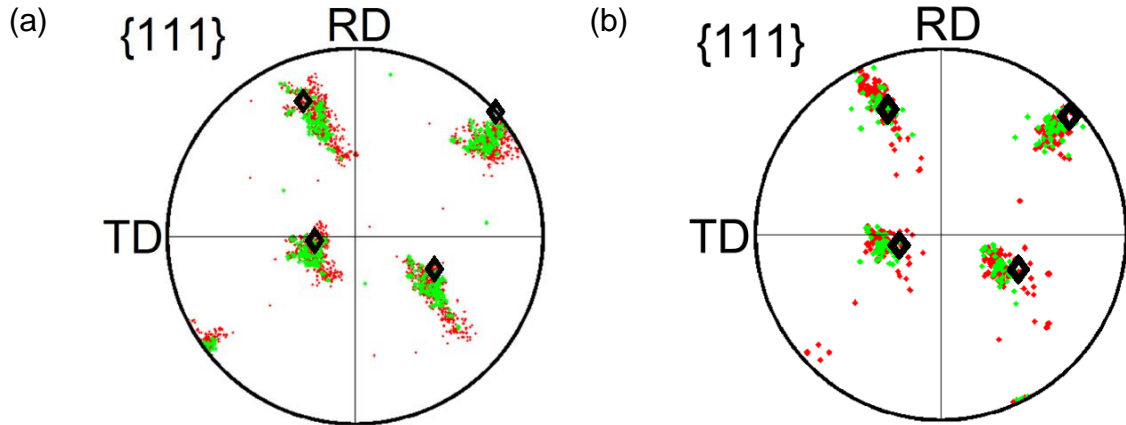
Figure 5.6: \{111\} pole figures showing the orientation relationships between nuclei and the matrix in the corresponding volumes in the deformed state before annealing: (a) nucleus No.1 and (b) nucleus No.3. The nucleus orientation is shown by large black diamond shaped markers. Red dots show the orientations in the deformed state for voxels identified as belonging to the nucleus after annealing, and green dots show voxels belonging to the 'cloud' around the nucleus volume, included to allow for the possible small sample misalignment when remounting the sample after the annealing. (b) is reproduced from article D.
