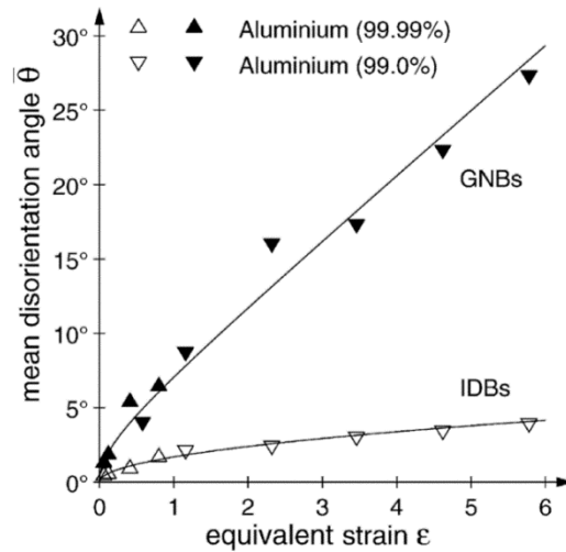
Figure 1.2: Evolution of the average misorientation angle across different types of boundaries (IDBs and GNBs) in aluminum during cold rolling. The triangles are the measured data in [50] and the full lines are fits of Eq. (12) in [48] to the experimental data from [50] for aluminum of two different purities (99.99%, 99.0%). Reproduced from [48].
