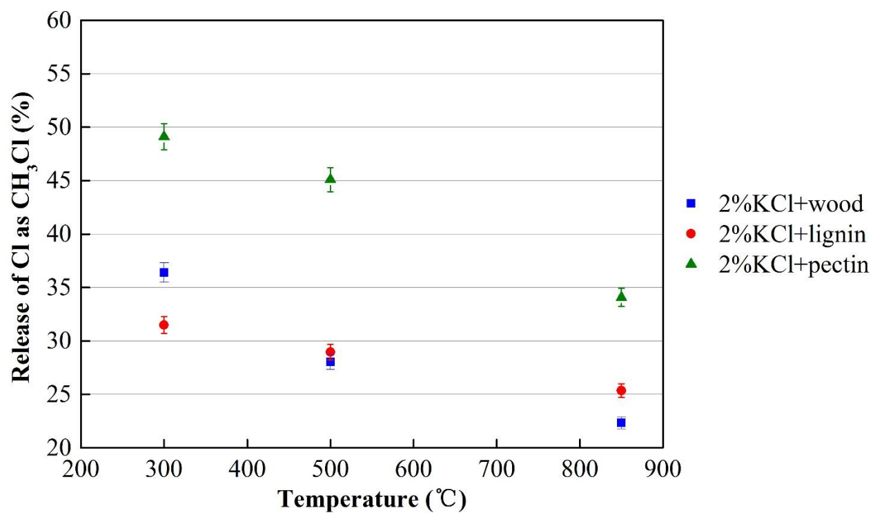
Figure 4 Influence of holding temperature on the release of Cl as CH 3 Cl (heating rate: 500°C/min).
