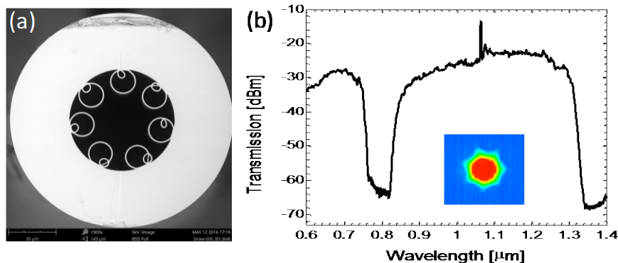
Fig. 1(a) SEM image of the fabricated 7-capillaries AR-HCF. (b) Measured transmission spectrum and near field mode profile obtained at 1064\text{ nm} .
