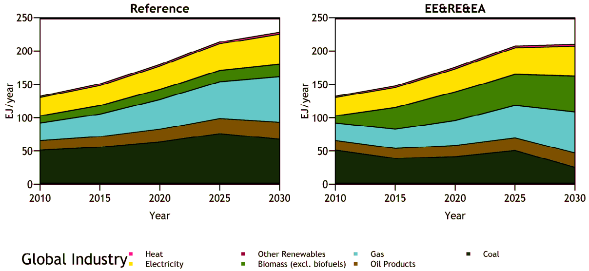
Figure 31. Global industry final energy consumption: Ref and EE+RE+EA scenarios.
