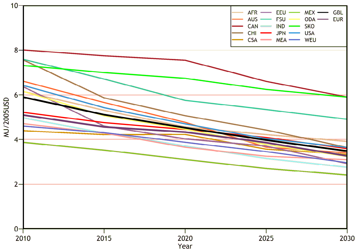
Figure 14. EIIIR from the EE+RE+EA scenario.
