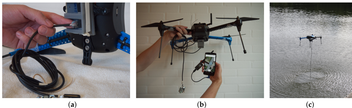
Figure 2. Operator-assisted flight: (a) A sensor (i.e., water thermometer) is mounted in the multi-socket and a small sketch in Arduino is written, (b) entire system with drone, sensor, smart-phone and antenna (c) flying manually over the lake to measure water temperature.
