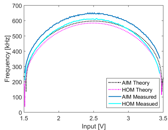
(b) Switch frequency
