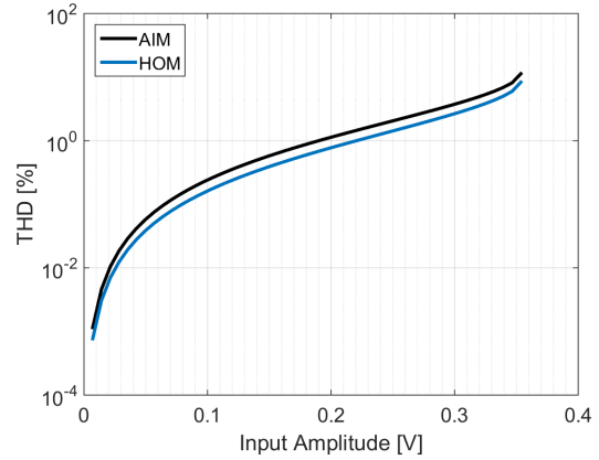
Fig. 8: Theoretical THD of both modulators
