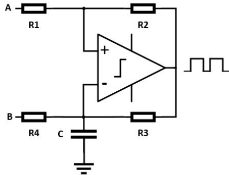
Fig. 3: Implementation of AIM and HOM
