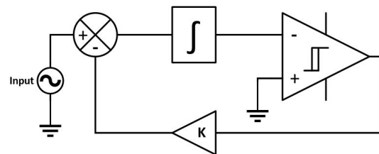
Fig. 2: Concept of the AIM
