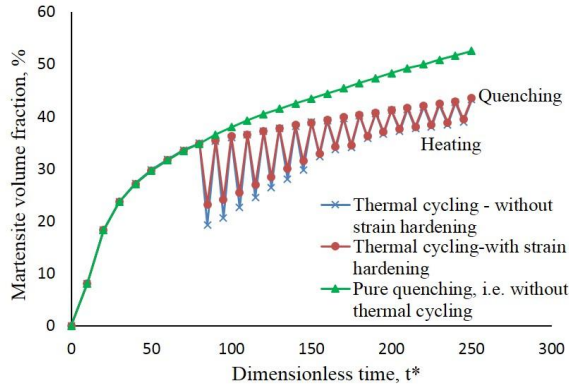
Figure 2: Variation in martensite volume fraction.
