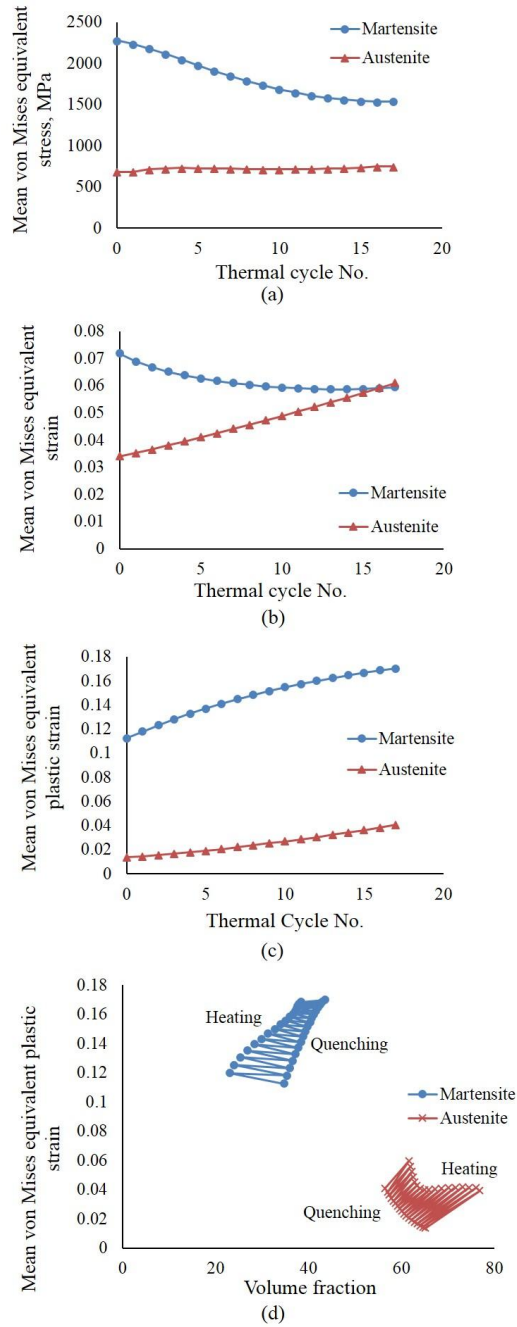
Figure 3: Variation of mean von Mises equivalent (a) stress (b) strain (c) plastic strain with thermal cycles (d) variation of mean von Mises equivalent plastic strain with volume fraction.
