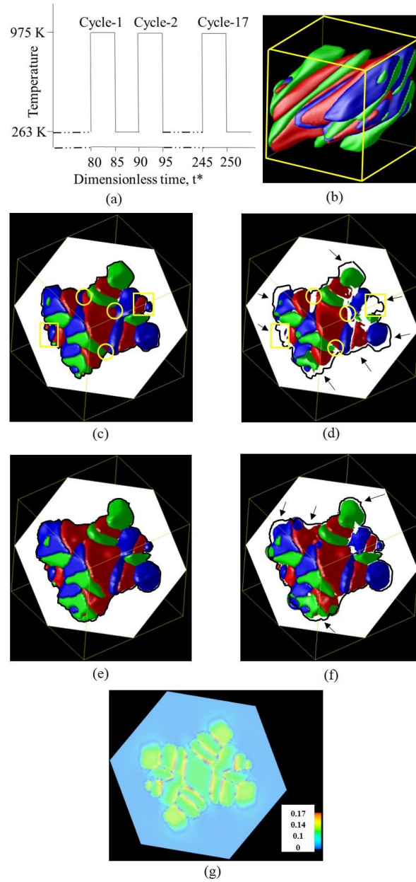
Figure 1: (a) Schematic of the simulated thermal cycling process. Microstructures at (b) t^* = 80 (side view) (c) t^* = 80 (top view) (d) t^* = 85 (e) t^* = 190 and (f) t^* = 195 and (g) von Mises equivalent plastic strain plot of the microstructure in (d). Martensite variants are shown in red, blue and green. Austenite on the (111)^\gamma plane is shown in white. Arrows point towards the areas where reversion occurs.
