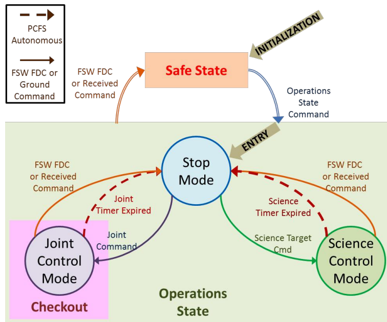
Figure 7. Pointing Control Flight Software mode transition diagram.
