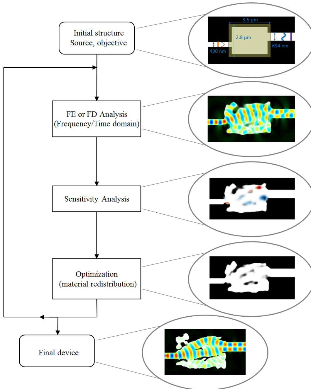
Figure 2.0.1: Schematic illustration of the concept of topology optimization. The squares in the center indicate a given step in the procedure while the ovals to the right contain corresponding design examples from the mode converter design presented in section 5.2. To the left the development of the same design is illustrated, to show what happens during the many iterations.
