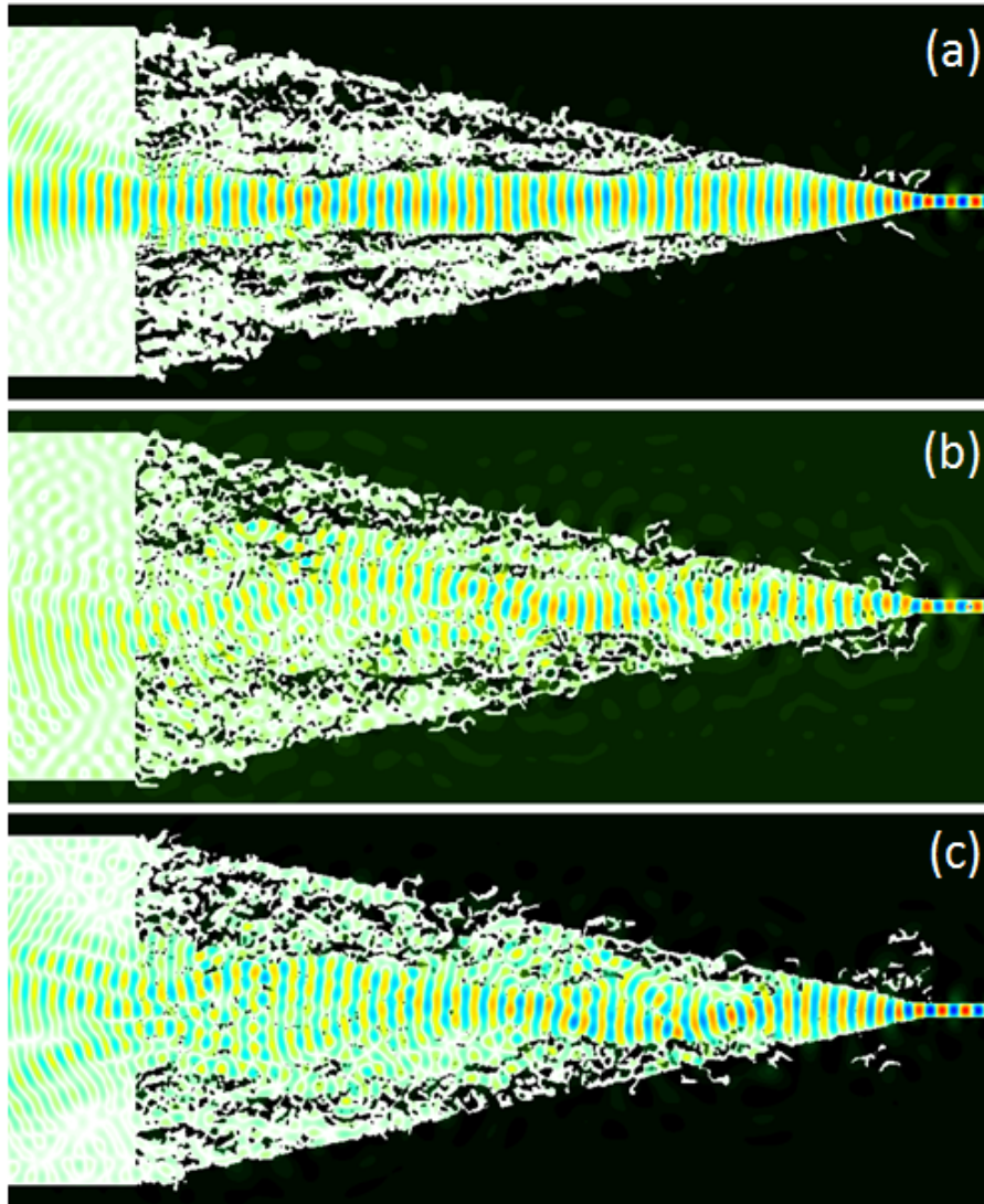
Figure 7.2.4: 3D optimized designs of a 27\ \mu\text{m} long taper along with H_z field simulations. The objective is placed in the wide waveguide and are of the pulse shape form. (a) Optimized design obtained from a propagation time from source to objective of 411\ \text{fs} , corresponding to the time from center to center in the unoptimized structures. (b) Increased delay time from source to objective, 500\ \text{fs} . (c) Design gained by having a non-constant time delay across the wide waveguide, introducing a delay at the center.
