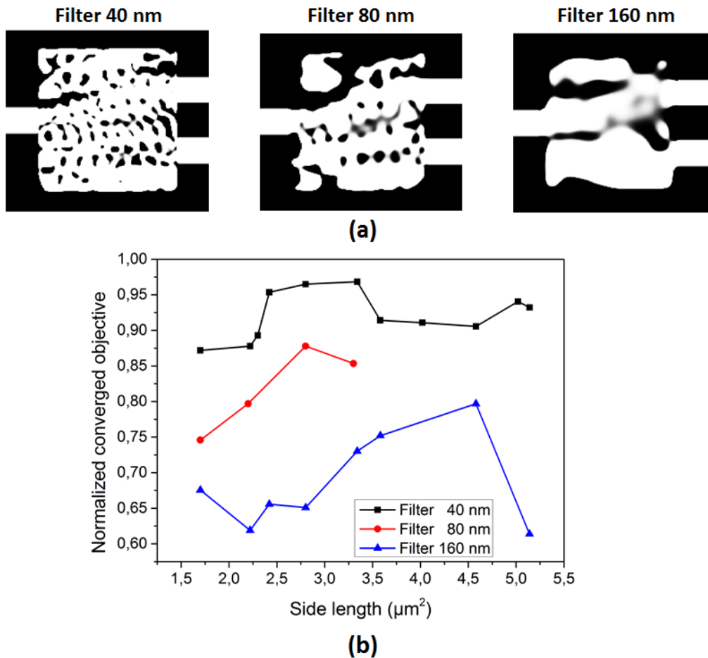
Figure 6.3.1: (a) Topology optimized wavelength multiplexers with symmetric waveguide positions and a footprint of 7.73 \mu\text{m}^2 optimized for three different filter sizes of 40 nm, 80 nm, and 160 nm respectively. (b) Normalized converged objective function value as function of design domain footprint shown for the three different filter radii.
