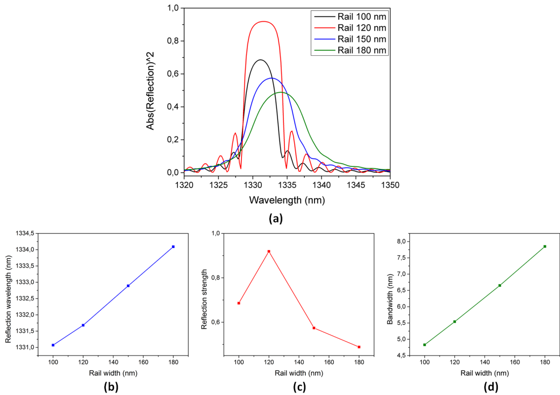
Figure 8.3.2: (a) Reflection spectra of the continuous width C-DBRs for various widths of the rail while other parameters are kept fixed at Angle = 45^\circ and Gap = 170 nm. (b-d) show the development of reflection wavelength, reflection strength and bandwidth as a function of the rail width, respectively.
