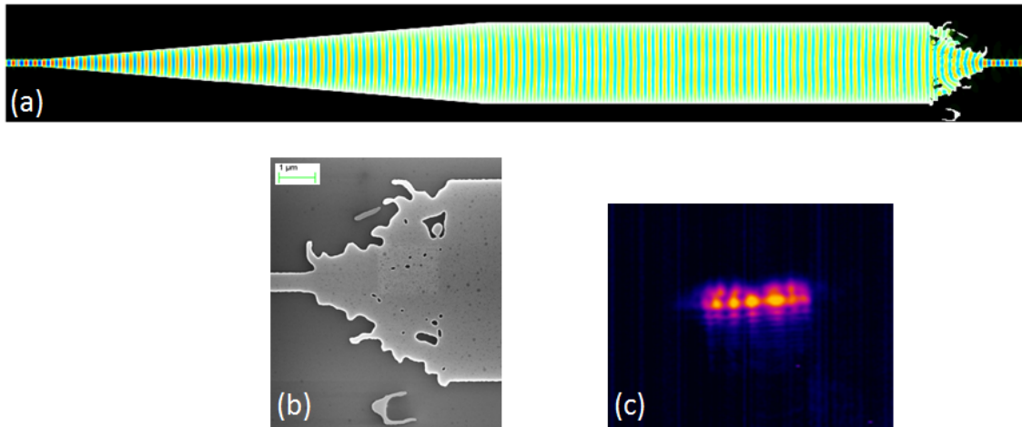
Figure 7.2.1: (a) Compact taper obtained from topology optimization on a 4.0\ \mu\text{m} region. A long leading taper has been introduced to obtain the \text{TE}_0 mode for the optimization. (b) Close up SEM image of the optimized region. (c) Mode profile of the light input in the narrow photonic wire and having traversed the optimized taper recorded at 1570\ \text{nm} .
