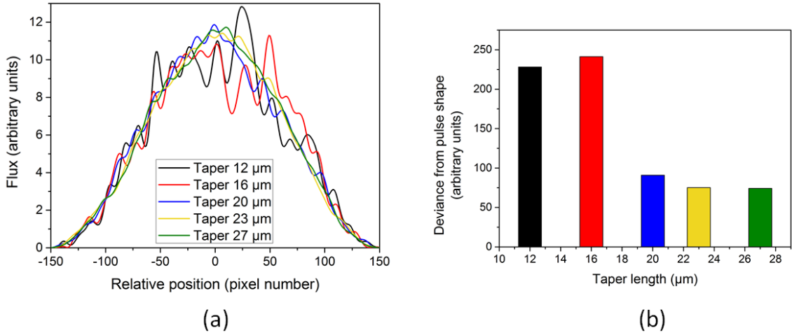
Figure 7.2.2: (a) Comparison of the simulated flux after optimization presented for numerous different tapering lengths. The design domain has the same width of 12.6 \mu\text{m} in all cases and the same length as the taper. During optimization the source was excited in the wide waveguide using the monotonous and symmetric profile exciter of figure 7.1.3. (b) A visualization of the deviation of the flux profiles of the optimized structures from that of the excited pulse. The plotted values are the integrals of the absolute values of the difference between the optimized and the intended pulse shape.
