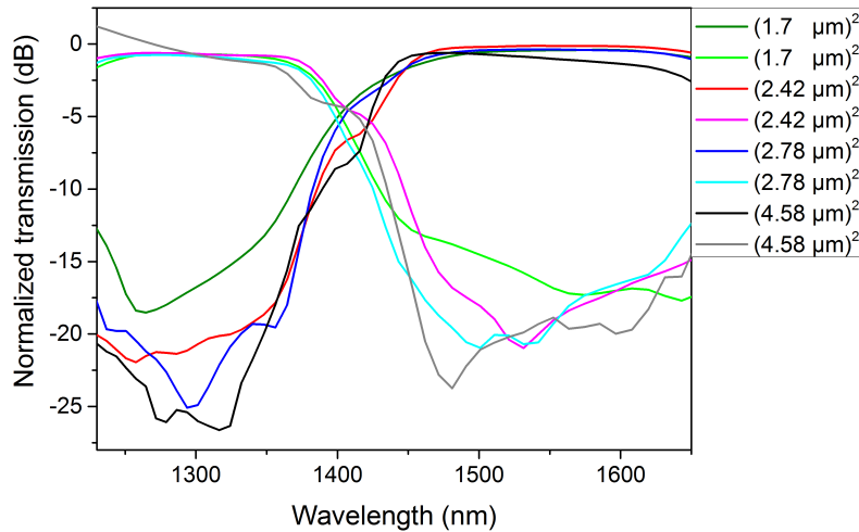
Figure 6.2.5: Spectra of the topology optimized wavelength multiplexers presented in figure 6.2.4(a). All spectra are normalized to the spectrum of the same source propagating through a straight waveguide.
