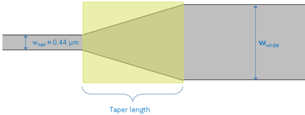
Figure 7.0.2: Sketch of the basis structure for the optimization of a compact taper. The narrow waveguide has a width of 0.440 \mu\text{m} while the width of the wide was varied to be around 6 \mu\text{m} and 12 \mu\text{m} respectively. In either case the design domain (yellow) covers the linearly tapered region the length of which was also changed throughout the various optimizations.
