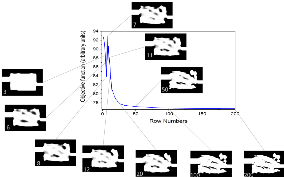
Figure 2.1.2: Illustration of the development of a design and its convergence. The objective function shows the overall convergence. The design is shown at choice points throughout the optimization (iteration number noted on the image) to illustrate the overall changes. In the beginning big changes occur in only a few iterations and large grey-scale areas are present. Towards the end the majority of what happens is refinement and a change to a black/white scale.
