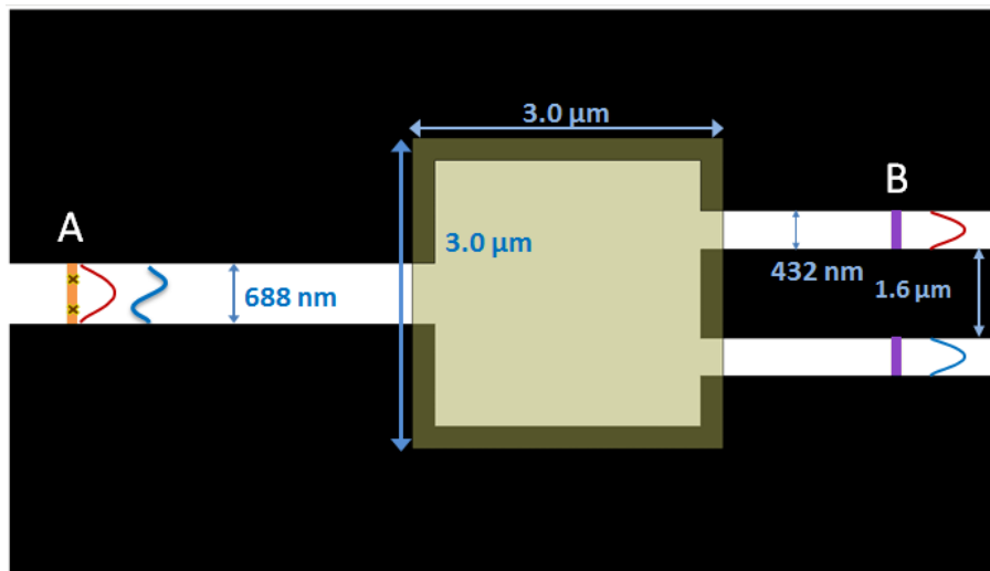
Figure 5.3.5: Example of the symmetric starting point structure for the 2-mode multiplexer working on TE_0 and TE_1 . Several variations were made with differing dimensions of the design domain (yellow), however the principle is the same. The orange bar in the left waveguide indicates the source position in the x direction and illustrates the excitation of the fundamental mode. The two brown crosses on top of it indicates the excitation of the first order mode using two point sources with opposite orientation. The objectives of the optimization are placed at the purple bars at position B. The resolution is 16 nm/pixel.
