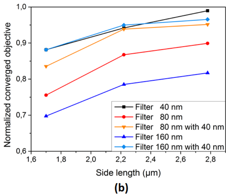
Figure 6.3.4: (a) Square design domain topology optimized wavelength multiplexers with asymmetric waveguides and a side length of 2.78\ \mu\text{m} for various filtering configurations. Top row has three different filter radii while the bottom row shows reoptimization using the top row structures as a starting point and applying a 40\ \text{nm} filter in the end. (b) Comparison of the performance quantified by the normalized converged objective value for the asymmetric multiplexer with various filter configurations.
