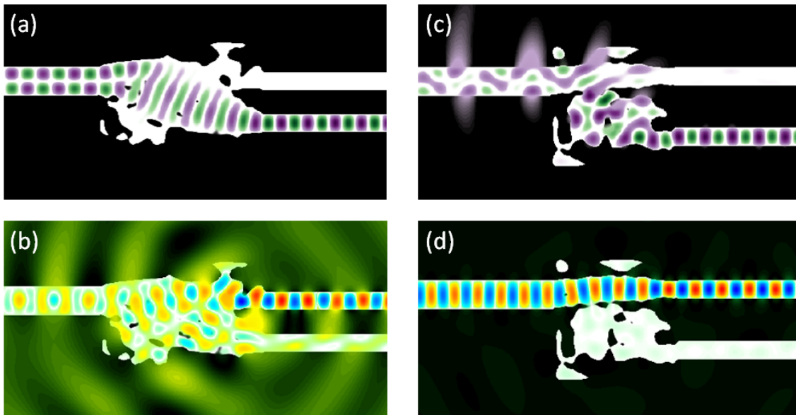
Figure 5.3.7: 2D FDTD simulations of the fields being multiplexed through two different attempted designs of a 2-mode multiplexer. (a) TE_1 and (b) TE_0 through a 2\ \mu\text{m} \times 3\ \mu\text{m} design. (c) TE_1 and (d) TE_0 through a 3\ \mu\text{m} \times 3\ \mu\text{m} design. Note that the size is not the only difference of the starting point, the waveguide positions are also key parameters for the designs. (a) and (d) were the best designs obtained for the two respective channels.
