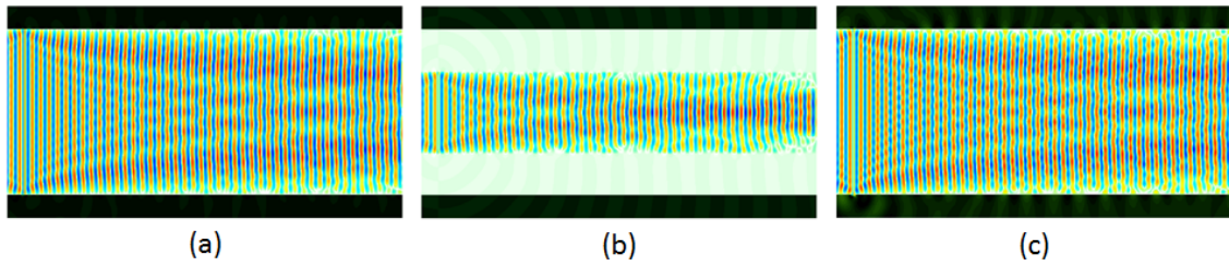
Figure 7.1.1: Attempts at exciting the TE_0 mode through placement of a single source with a uniform intensity distribution in the wide leading region of a tapering structure. (a) A single source extending through the entire width of the waveguide. (b) A single source with a width half that of the waveguide. (c) A single source which extends beyond the edges of the waveguide.
