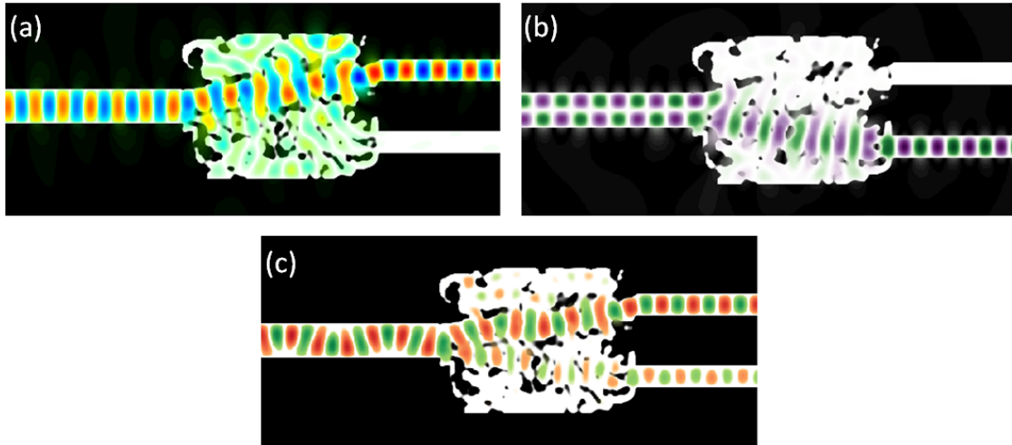
Figure 5.3.6: 2D FDTD simulations of the fields through a 2D optimized 2-mode multiplexer with a footprint of 3\ \mu\text{m} \times 3\ \mu\text{m} . (a) The TE_0 field, (b) the TE_1 field, and (c) the two fields excited simultaneously illustrating the multiplexed field which is more difficult to qualitatively evaluate.
