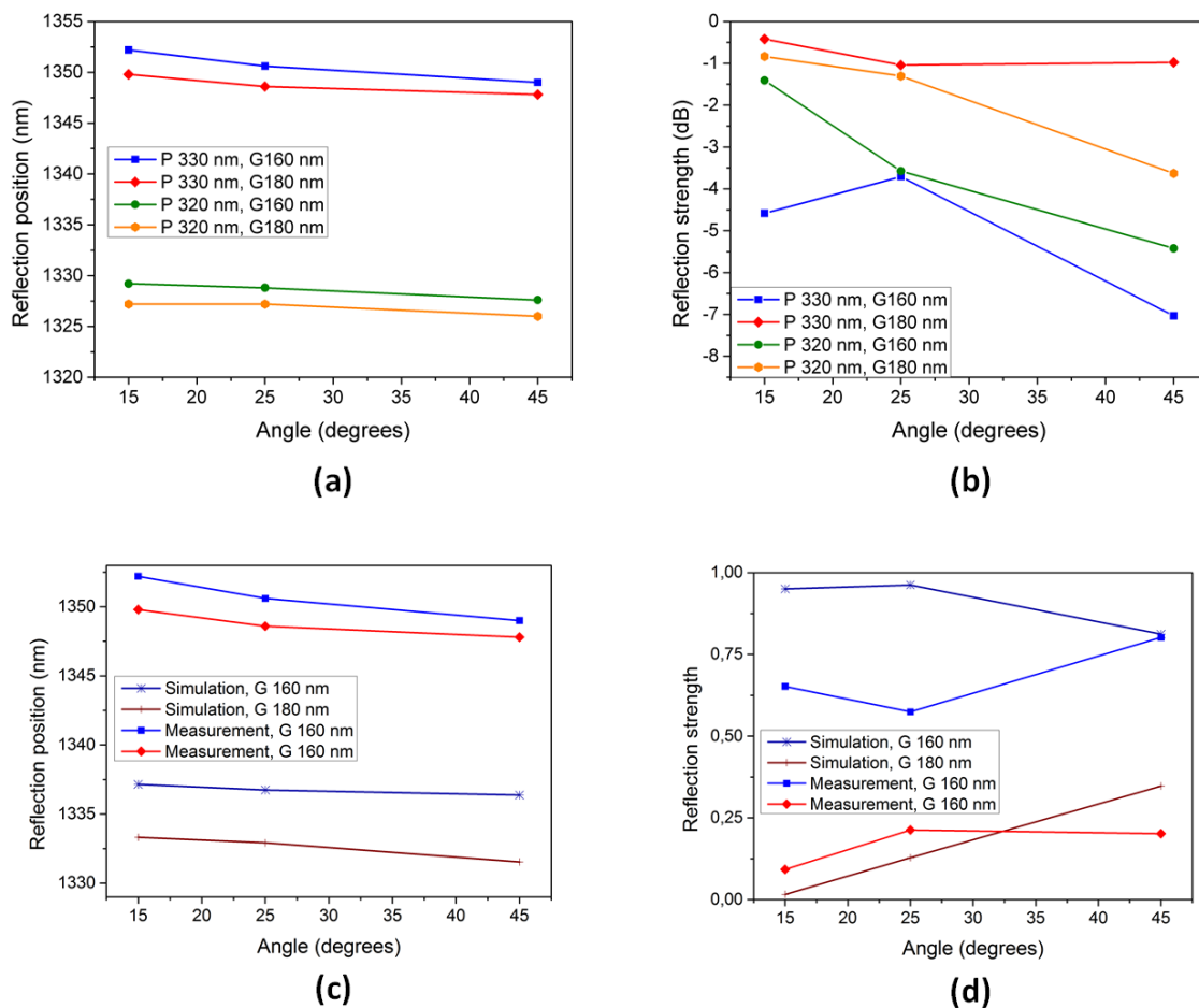
Figure 8.3.12: Development of (a) reflection position and (b) reflection strength as a function of the angle for a continuous width cladding modulated grating with a central waveguide width of 320 nm and a rail width of 150 nm. Results presented for two sets of periods and two different gaps. (c,d) Direct comparison of the simulated and experimental results or the P = 330 nm datasets.
