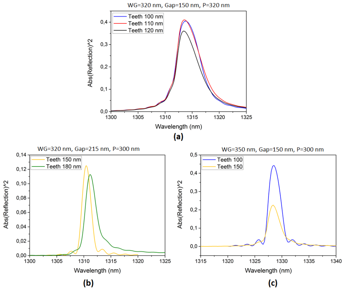
Figure 8.2.2: Simulations of the reflection from the continuous step index gratings when the tooth size, that is the depth of the wedge, is altered. Within each graph all other parameters than the wedge depth are fixed and the values are specified above. Gap width, width of the center waveguide and the period have been altered between subfigure (a), (b) and (c).
