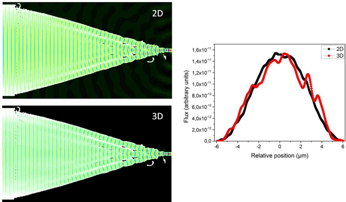
Figure 7.2.3: 2D optimized design for a 20\ \mu\text{m} long taper with the field simulated in 2D and 3D respectively. The simulated flux after conversion is shown for a direct comparison of the devices.
