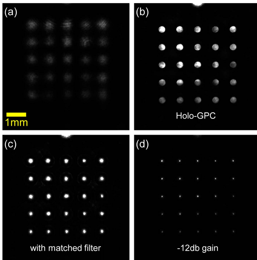
Fig. 6. A 5 \times 5 holographically diffracted Gaussian spot array (a) shaped into circles via Holo-GPC (b), then converted into intense spikes (c) via matched filtering. To reduce the saturation (d), the camera gain had to be 12db lower.
