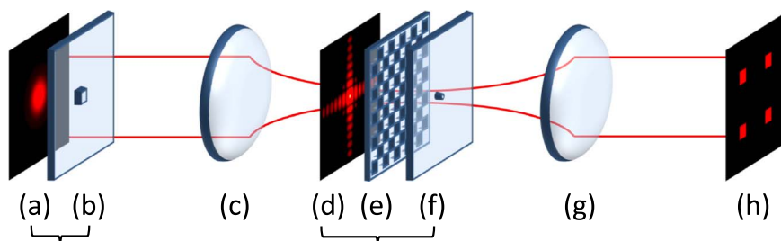
Fig. 2. Holo-GPC setup. Compared to standard GPC, a hologram (e) is placed in addition to the PCF at the Fourier plane of the first lens. For practical implementations, the hologram is typically encoded on an SLM, and the sizes of the input beam, phase mask, PCF and focal lengths have to be adjusted. The second lens (g) optically Fourier transforms the light that is altered by the hologram and PCF to get a distributed output consisting of speckle-free contiguous shapes.
