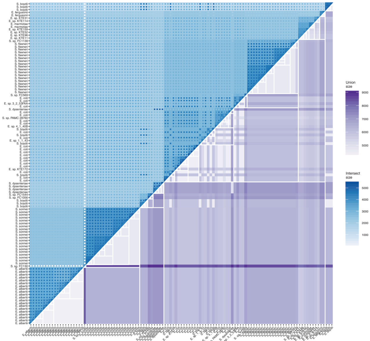
Fig. 5. A dendrogram inspired heatmap showing pairwise intersection and union sizes. The hierarchical clustering has been overlaid with white lines on top of the union sizes while the set family intersection size for each cluster has been indicated as a backdrop color below the pairwise intersections. The contrast between the set family intersection sizes and the pairwise intersection size is indicative of how well the hierarchy describe the relationship between the two sets
