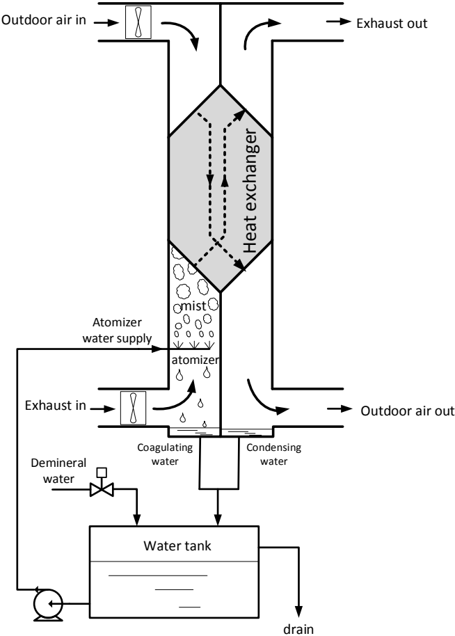
Figure 1. Principle of the developed total heat recovery unit.
