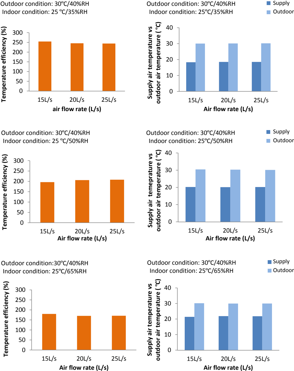
Figure 3. The measured temperature efficiencies and temperatures of supply and outdoor air at the three levels of airflow rate. The experiment was conducted at the simulated extreme Copenhagen summer climate and three air-conditioned indoor climate.
