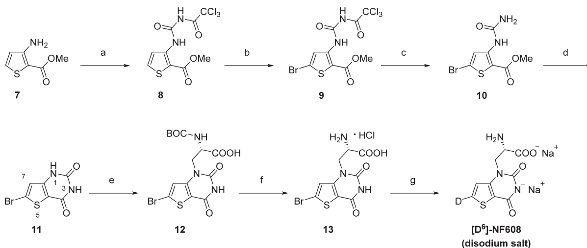
Scheme 2 Synthesis of key 6-bromo precursor 13 and incorporation of deuterium to give [\text{D}^6] -NF608. Reagents and conditions. (a) Trichloroacetyl isocyanate, THF, 0 °C to rt, 2 h, 93%; (b) \text{Br}_2 , acetic acid, 0 – 80 °C, overnight, 69%; (c) 2 N \text{NH}_3 in methanol, 0 °C to rt, 30 min, 89%; (d) tert -BuOK, DMF, rt, overnight, 95%; (e) NaH, DMF, 0 °C to rt, then lactone 2 in DMF, 0 °C to rt, 18% (f) 2 M aq HCl, 50 °C, 1 h, 94% (g) \text{D}_2 (g), Pd/C, NaOH, \text{H}_2\text{O} , rt, overnight, 57%.
