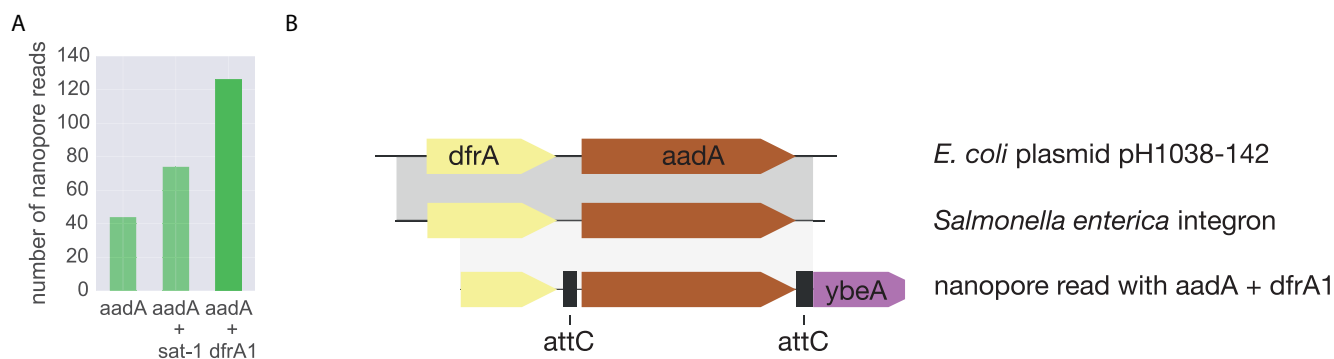
Figure 6. (A) Example of CARD genes found in the nanopore dataset that were plated on spectinomycin. Of the 244 nanopore reads that were recovered on spectinomycin, all contain the aadA , which encodes an aminoglycoside nucleotidyltransferase known to confer resistance to spectinomycin. In 126 reads aadA is flanked by dfrA1 , which confers resistance to trimethoprim and in 74 reads aadA is flanked by sat-1 which confers resistance to streptomycin. The genes sat-1 and dfrA1 do not confer known resistance to spectinomycin and are thus co-selected with aadA . (B) Alignment against the NT database of the longest corrected nanopore read of the 126 reads containing aadA and dfrA obtained from functional selection on spectinomycin. The corrected nanopore read shares 99% sequence identity with the two top scoring hits in the NT database: (light gray) integron from Salmonella enterica subsp. enterica serovar (GenBank: HQ132378.1) and the E. coli plasmid pH1038-142 (genbank: KJ484634) described by Wang et al. (38). The attC region is a repeat sequence which typically flanks a resistance cassette, dfrA encodes a dihydrofolate reductase known to confer resistance against trimethoprim, aadA is an aminoglycoside nucleotidyltransferase known to confer resistance to spectinomycin and ybeA (also known as orfX ) which is a pseudocassette and present as conserved 3' fragment in class 2 integrons (36).
