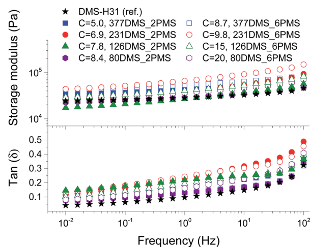
Fig. 3 The storage and \tan(\delta) of cross-linked PDMS-PPMS copolymers at 23 °C; C is in 10^{-4} mol g -1 .
