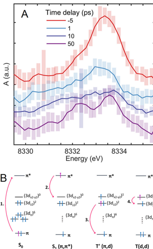
Figure 4. (A) XANES scans in the 1s \rightarrow 3d region (Figure 2A, E0), 5 pt smoothed and with the rising XANES edge background subtracted. Offset in A(a.u.) for clarity. (B) 3d-orbital occupations of electronic states in the NiTMP relaxation pathway resulting from: (1) excitation of the porphyrin macrocycle, (2) charge transfer from the macrocycle \pi^* orbital to the Ni metal center, (3) reverse charge transfer from Ni to the macrocycle via relaxation of a 3d_{z^2} electron into the \pi hole, (4) relaxation of the 3d_{x^2-y^2} electron into the 3d_{z^2} to recover the ground state d-orbital configuration. Note naming convention w.r.t. spin state. 51
