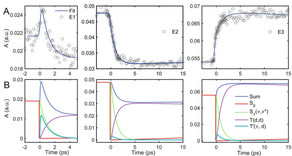
Figure 3. (A) Single-energy delays scans at (left to right) 8337, 8338.5, and 8341 eV with fits to kinetic model (1) (dark blue line). (B) Decomposed signal contributions from each electronic state accounted for in the fit of model (1) to the delay scans at (left to right) 8337, 8338.5, and 8341 eV determined by numerical integration of the rate expression for each species, in this case for the assignment \tau_1 = 1.0 ps, \tau_2 = 0.08 ps ( <300 fs). The resulting total signal for each energy (dark blue) was fit to the delay traces.
