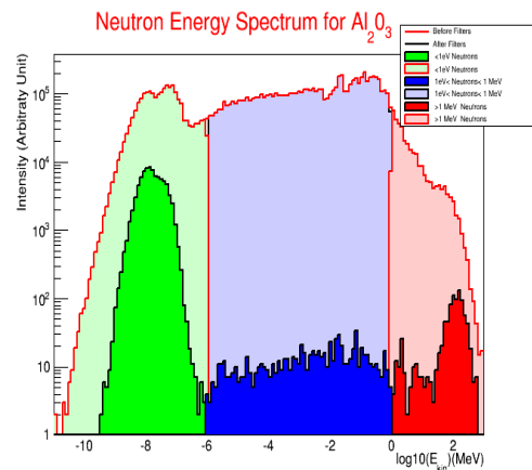
(f) Neutron spectrum before and after the filter for 3 blocks of 15 cm.
