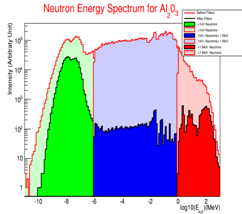
(d) Neutron spectrum before and after the filter for 2 blocks of 10 cm.
