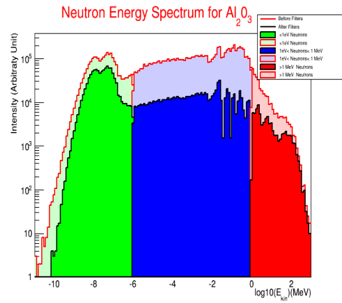
(b) Neutron spectrum before and after the filter for 1 block of 5 cm.
