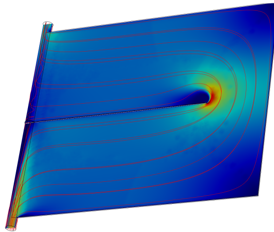
Figure 2. Flow field in the draw channel of one unrolled envelope in FO operation: Through implementing a baffle across \sim 3/4 of the length of the envelope and pressurizing the feed tube inlet, a channel is created and the spiral wound membrane module can be operated in FO.
