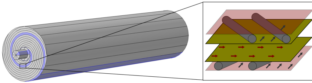
Figure 1. Sketch of the geometry of the spiral wound membrane module, with the actual computational domain highlighted in blue and a detailed sketch of the computational domain. The green surfaces are the respective membranes of the envelope. Between them, the flow field of the permeate (RO) or draw solution (FO) is indicated by the red arrows. Outside the envelope half of the feed channel is added to either side of the envelope. The grey cylinders represent the feed spacers and the black arrows indicate the feed solution flow field. The red-transparent surfaces are the crucial part of the model: They represent a pair of periodic boundaries in the middle of the feed channel.
