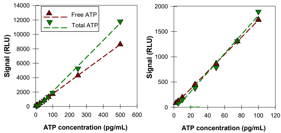
Figure 2. Calibration curves for free and total ATP for a wide (left panel) and low ATP concentration range relevant for drinking water systems (right panel).
