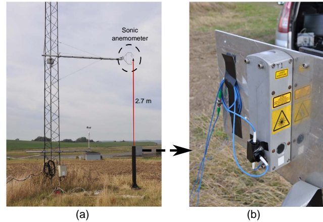
Figure 4. Field campaign at Risø campus of the Technical University of Denmark. (a) shows the position of the ICDL's output antenna with respect to the sonic anemometer. (b) is an expanded view of the mounting plate for the antenna, viewed from the backside of the plate seen in (a).
