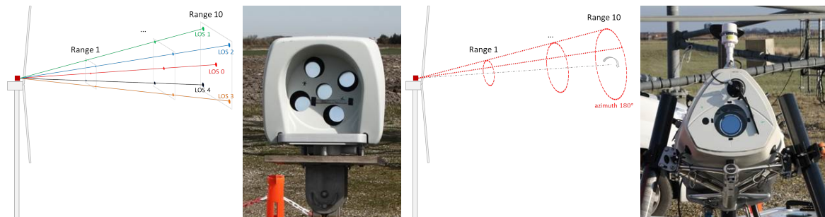
Figure 1. Two wind profiling nacelle lidar examples: 5-beam Avent Demonstrator (left) and Zephir Dual-Mode (right).
