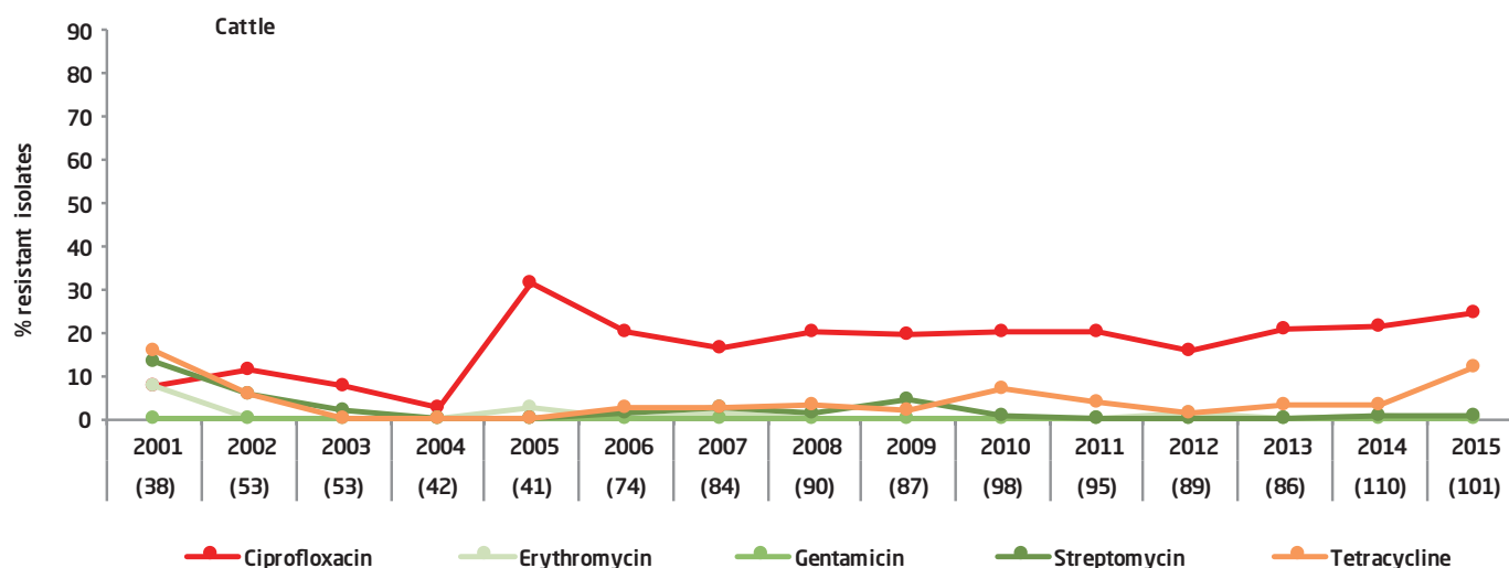
Figure 6.5. Resistance (%) in Campylobacter jejuni from cattle, Denmark
