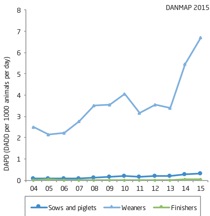
Figure 4.5. Consumption of colistin in finishers, weaners, sows and piglets, Denmark
