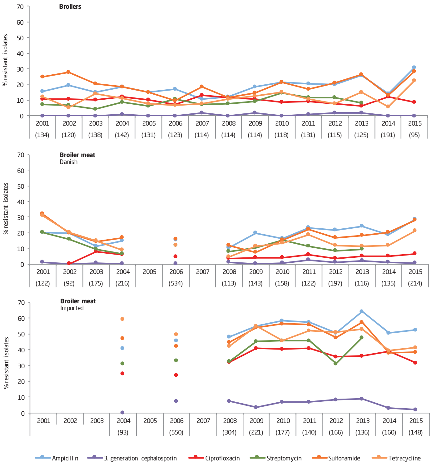
Figure 7.4. Resistance (%) in Escherichia coli from broilers and broiler meat, Denmark
