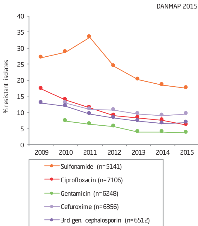
Figure 8.8. Resistance (%) in Klebsiella pneumoniae urine isolates from humans in hospitals, Denmark
