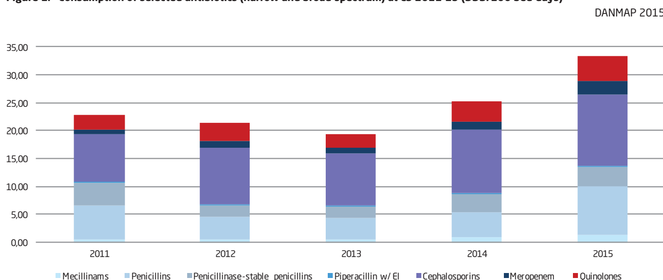
Figure 1. Consumption of selected antibiotics (narrow and broad-spectrum) at LS 2011-15 (DDD/100 bed-days)
