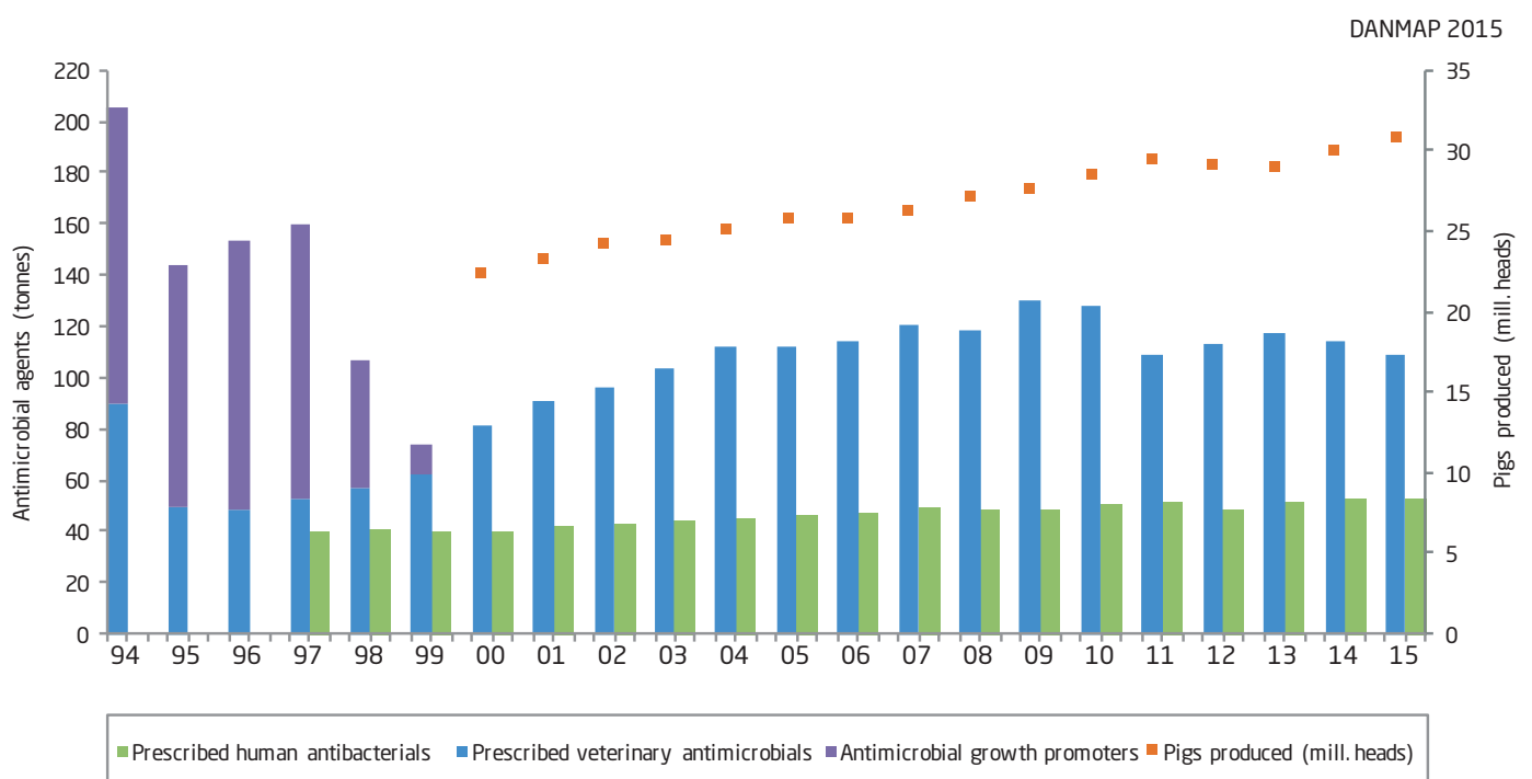
Figure 4.1. Prescribed antimicrobial agents for humans, and for all animal species, including the number of pigs produced, Denmark
