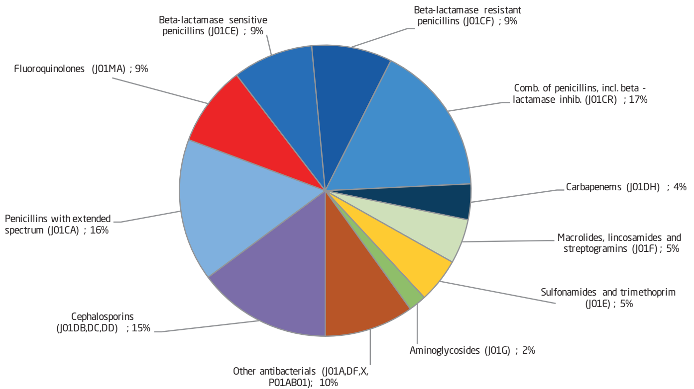
Figure 5.13. Distribution of the total consumption of antimicrobial agents in somatic hospitals, Denmark
