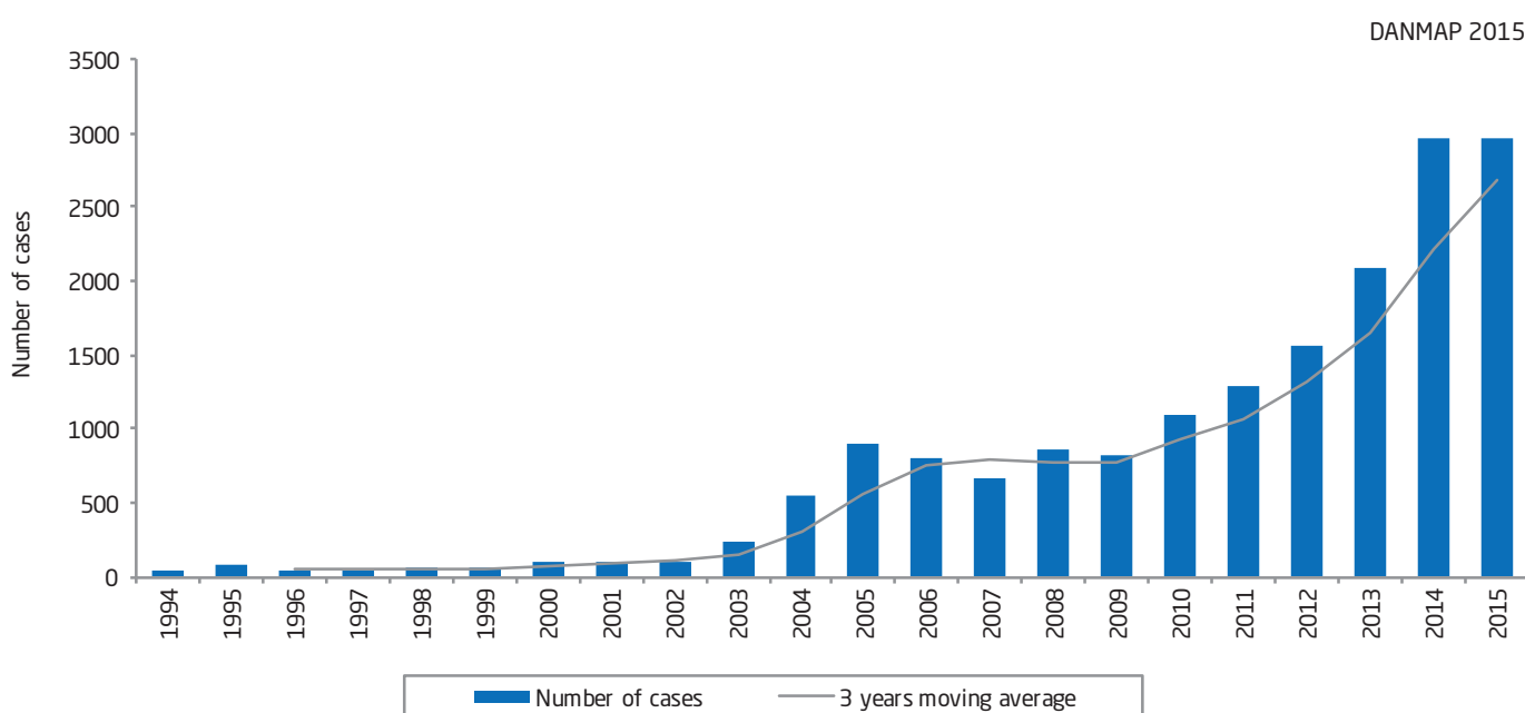
Figure 8.13. Number of methicillin-resistant Staphylococcus aureus cases, with a three years moving average, Denmark
