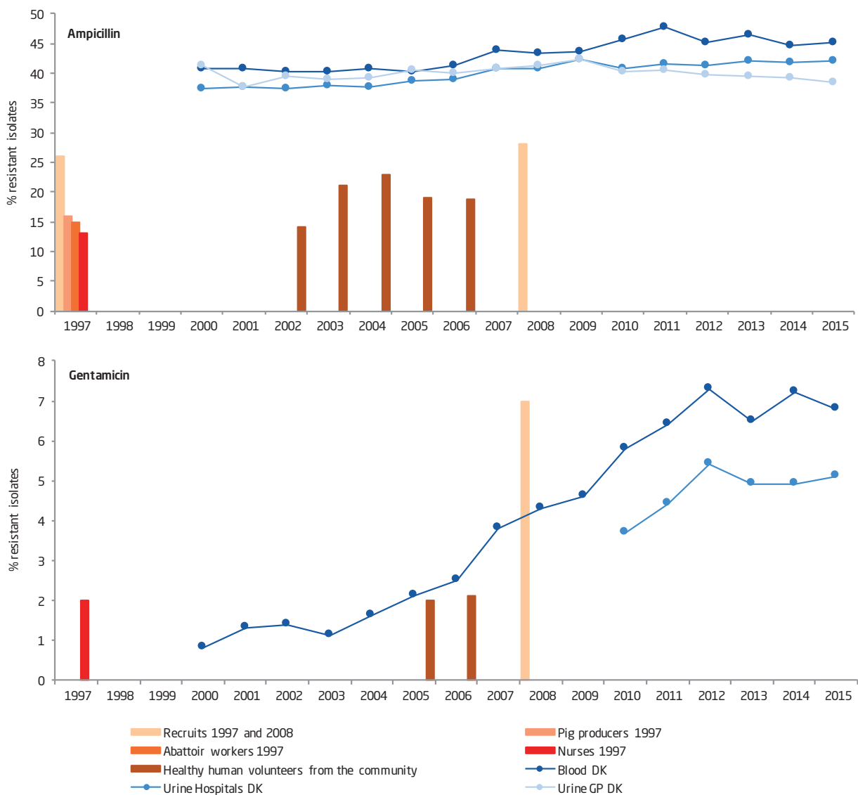
Figure 1. Resistance (%) to ampicillin, ciprofloxacin, gentamicin and 3rd generation cephalosporins in human E. coli clinical isolates and from the intestinal flora of different population groups
