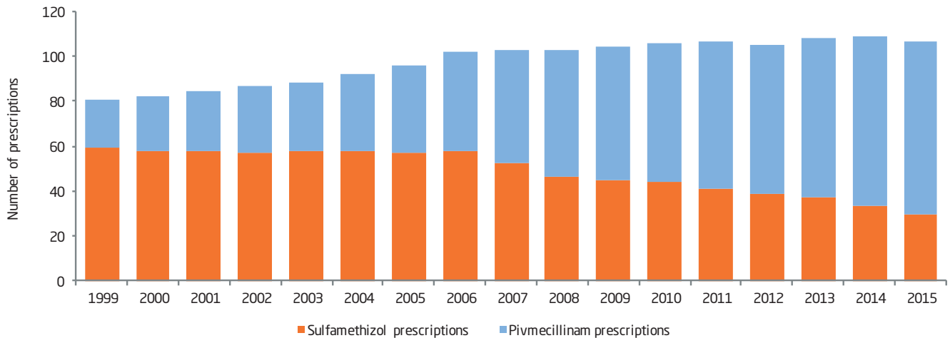
Figure 5.9, number of prescriptions for women treated for urinary tract infection, 1999 - 2015
