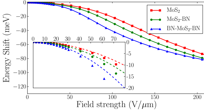
Figure 6.3: Exciton Stark shift in the MoS 2 based structures as a function of field strength calculated through complex scaling. Inset: the shift predicted by our simple hydrogenic model (dashed lines) agrees well with the complex scaling results for small fields.
