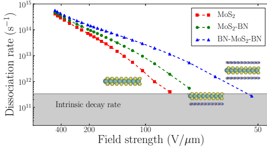
FIG. 3. The dissociation rate of an exciton in the \text{MoS}_2 layer as a function of in-plane field strength for the three different structures. The intrinsic decay rate spans between the defect-assisted fast decay of the excitons of 2–5 ps (upper limit) and the much slower radiative recombination of the excitons at room temperature (lower limit).
