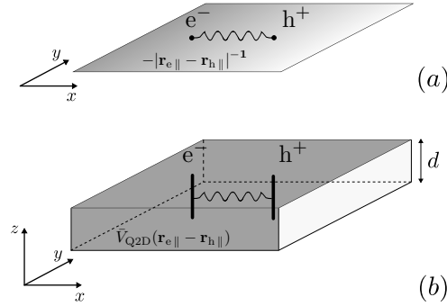
Figure 4.3: Sketch of the Coulomb interaction between (a) point-charges in a 2D plane and (b) quasi-2D point-charges, i.e. lines of charge extending along the thickness of the material.
