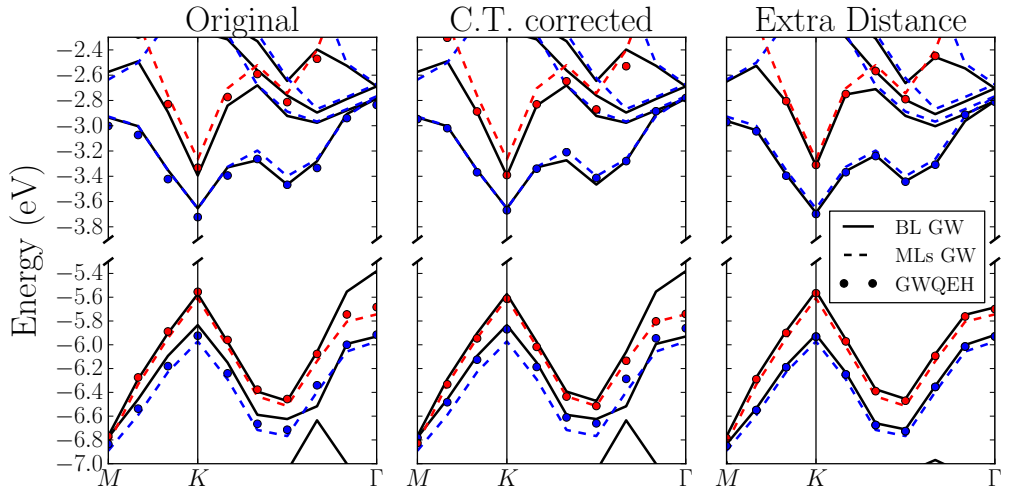
Figure 3: Comparison of the GWQEH method to G_0W_0 calculation for the lattice-matched bilayer. Left panel: reference calculation. Central panel: GWQEH bands are shifted upwards for MoS 2 and downwards for WSe 2 to account for the charge transfer. The values of the shifts are extracted from the comparison between the isolated layers and bilayer LDA calculations. Right panel: the layer separation is artificially increased by 3Å. With the extra distance we expect the effect of charge transfer and hybridization to be completely negligible. The isolated layer bands are reported in all the panels as reference. As usual blue is used for MoS 2 and red for WSe 2 .
