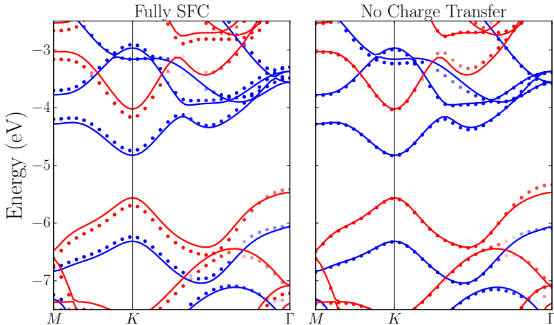
Figure 2: Left panel: bands for strained MoS 2 /WSe 2 bilayer (circles) and constituent monolayers (continuous lines). Here the charge transfer effect manifests as constant shift in opposite direction for MoS 2 (in blue) and WSe 2 (in red). Right panel bands for the same systems but for the bilayer the Hartree potential is not updated self-consistently. Keeping the Hartree potential fixed to the one of the isolated layers prevent charge transfer and therefore bilayer and monolayers bands coincide as long as hybridization is negligible. Hybridization is present around \Gamma .
