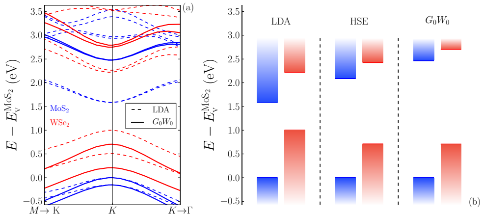
Figure 5.9: Panel (a): LDA and G_0W_0 band structure for the freestanding MoS 2 and WSe 2 layers. Only the portion of the BZ around the K -point is shown. Panel (b): comparison of the LDA, HSE (HSE06) and G_0W_0 band edges. We chose the top of the valence band in MoS 2 as reference energy to align the bands because of the uncertainty of the G_0W_0 vacuum levels. Spin-orbit effects are included in the calculations.
