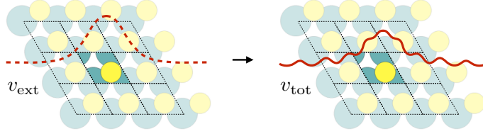
Figure 3.2: Illustration of the local field effects in a periodic system.
