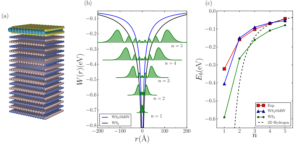
Figure 5.5: Excitonic Rydberg series in supported \text{WS}_2 . Panel (a): \text{WS}_2 supported on a hBN substrate. Panel (b): screened electron-hole interaction energy in the supported (blue line) and free standing (black line) \text{WS}_2 . The same panel shows the radial probability distribution, r|F(r)|^2 , of the first five excitonic states. The normalization is arbitrary. Panel (c): The Rydberg series calculated with the QEH for freestanding \text{WS}_2 (green) and \text{WS}_2 on hBN (blue) are compared to the experimental data from Ref. [95] for \text{WS}_2 on \text{SiO}_2 (red). The hydrogenic Rydberg series obtained for a constant \epsilon = 1.7 is also displayed for reference.
