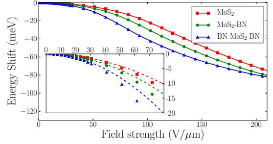
FIG. 4. The Stark shift in the \text{MoS}_2 heterostructures. The inset shows the shift for small fields, along with the shift predicted for a 2D hydrogen atom with an effective dielectric constant \epsilon_{\text{eff}} ; see Eq. (4).
