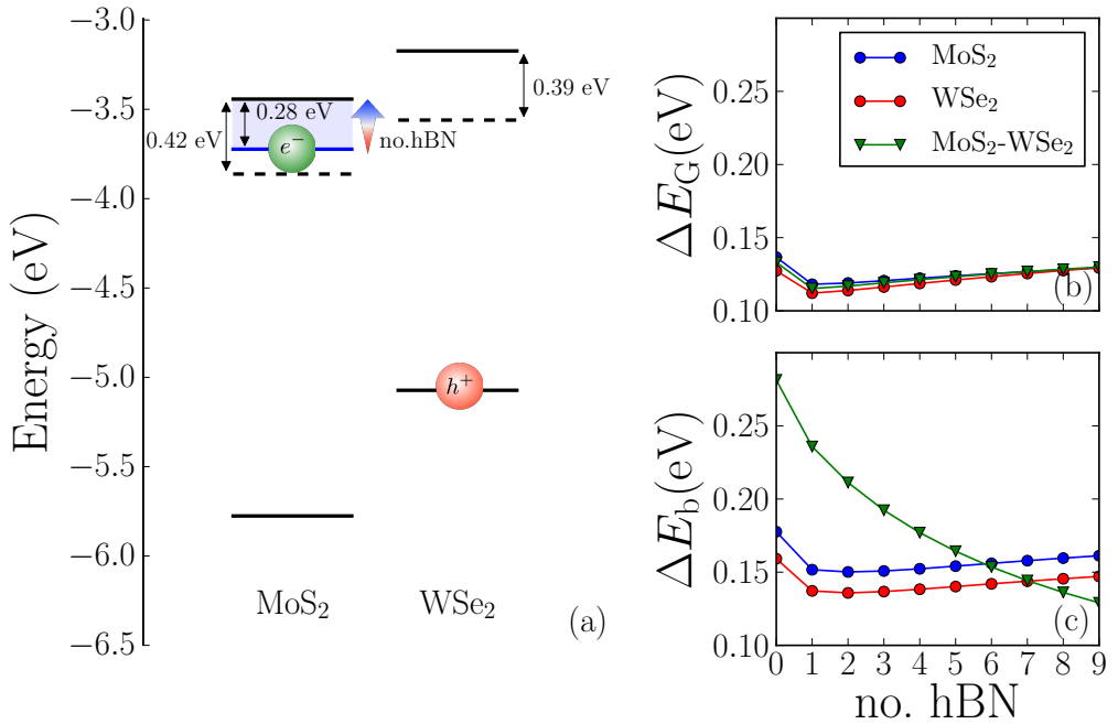
Figure 5: (a) Band alignment diagram for bilayer MoS 2 /WSe 2 calculated within the G_0W_0 -QEHA approximation (see text for details), along with lowest intra and inter-layer excitonic levels for bilayer MoS 2 /WSe 2 . The shaded region and the arrow shows that the interlayer exciton binding energy decreases with an increasing number of intercalating h-BN. Variation in intra and interlayer gaps (b) and exciton binding energies (c) as a function of intercalated BN layers.
