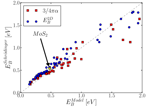
FIG. 1. Exciton binding energies of 51 transition metal dichalcogenides calculated as the lowest eigenvalue of Eq. (2) (vertical axis) and the model result Eq. (5) (horizontal axis). We have indicated the well-known example of MoS 2 .
