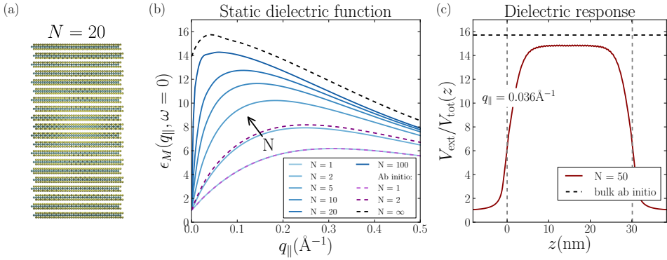
Figure 5.2: Panel (a): Cartoon of the MoS 2 multilayers. Panel (b): Dependence of the macroscopic static dielectric function \epsilon_M(\mathbf{q}_{\parallel}, \omega = 0) on the number of MoS 2 layers N . The QEH dielectric function converges towards the bulk ab-initio result for large N . Panel (c): Effective local dielectric function, defined as V_{\text{ext}}/V_{\text{tot}}(z) , meaningful for the screening of constant external potential across a N = 50 layers stack. The external potential is proportional to e^{i\mathbf{q}_{\parallel} \cdot \mathbf{r}_{\parallel}} in-plane direction, with \mathbf{q}_{\parallel} = 0.036 \text{\AA}^{-1} .
