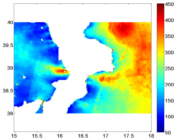
Fig. 3. Wind power density E ( Wm^{-2} ) from SAR, offshore the central area of the Calabria region. Period: 2002-2012. We note that offshore the northern end of the Santa Eufemia Gulf the wind speed is higher than offshore at the southern end in front of Vibo Valentia due to the channelling effect of the East-west oriented valley of the Marcellinara Gap.
