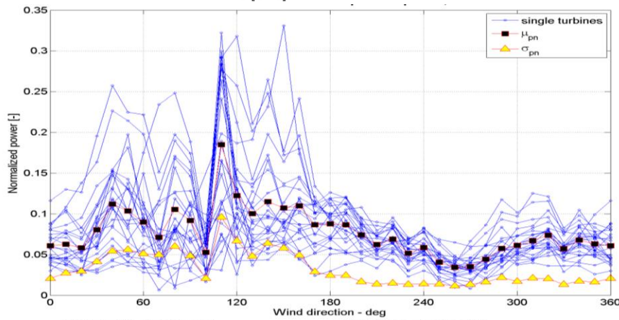
Figure 12: Normalized sector-wise mean power for each wind turbine. Furthermore, the figure includes the normalized and average park power production ( \mu_{PN} ) and standard deviation ( \sigma_{PN} ).
