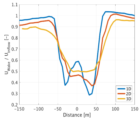
Figure 6: The horizontal wind speed profiles across the wake sector demonstrates a speed reduction at hub height - 1D, 2D & 3D downstream.
