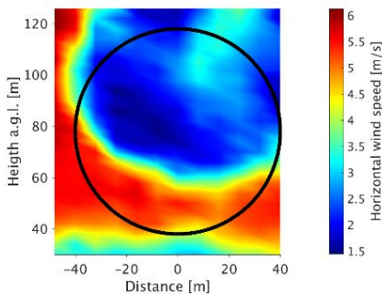
Figure 9: Horizontal wind speed distribution across the rotor disc, where the wake has been lifted - UP.
