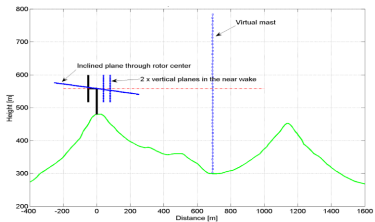
Figure 4: Measurement setup for the single wake measurement. The dashed 4^\circ inclined dashed line illustrates the diamond long range scanning plane through the hub. The short vertical lines behind the rotor illustrates the short range plane.
