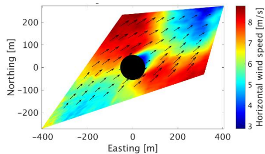
Figure 10: Horizontal wind speed distribution at hub height around a wind turbine, for a SHORT wake length.
