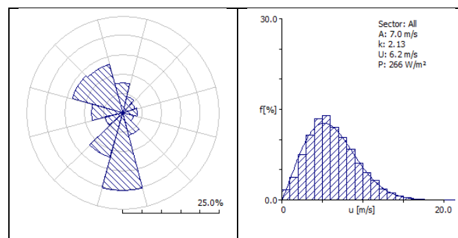
Figure 3: Wind climate at the WF measured during 2012 at hub height - recorded before the wind turbine installation.
