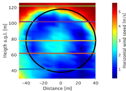
Figure 7: Horizontal wind speed distribution across the rotor disk - 1D downstream from the rotor disk. The wind speed distribution is recorded with the short-range WindScanner. DOWN
