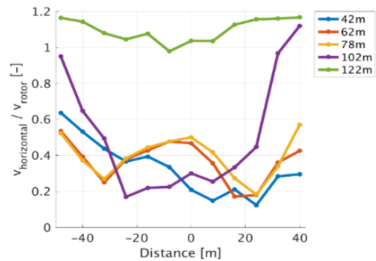
Figure 8 Horizontal wind speed profiles across the wake at 5 heights including hub height (78 m) - 1D downstream
