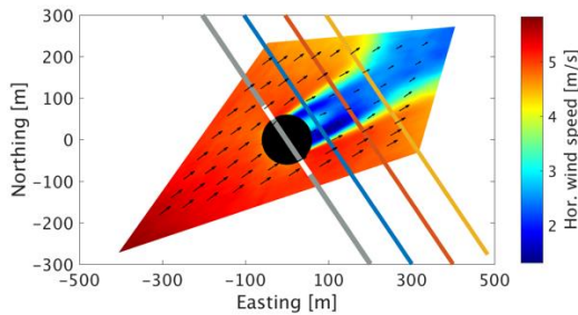
Figure 5: Horizontal wind speed distribution at hub height around a wind turbine, located on a NW-SE oriented ridge with a LONG wake sector.
