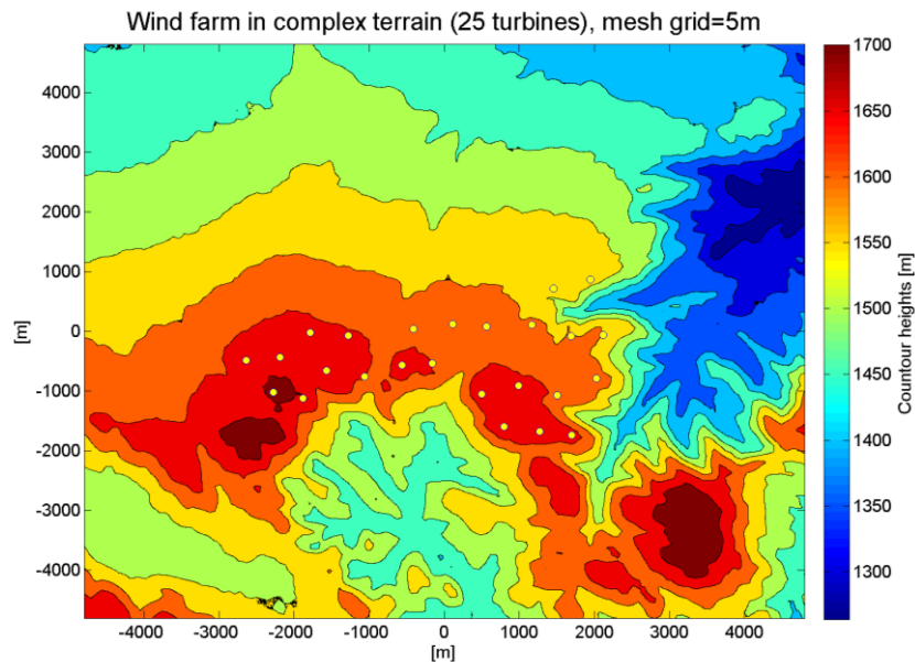
Figure 2: Wind farm landscape contour plot including location of 25 wind turbines (the white circles represent the wind turbines).
