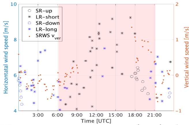
Figure 11: Diurnal cycle of the vertical wind speed and an indication of the wind turbine wake movement.
