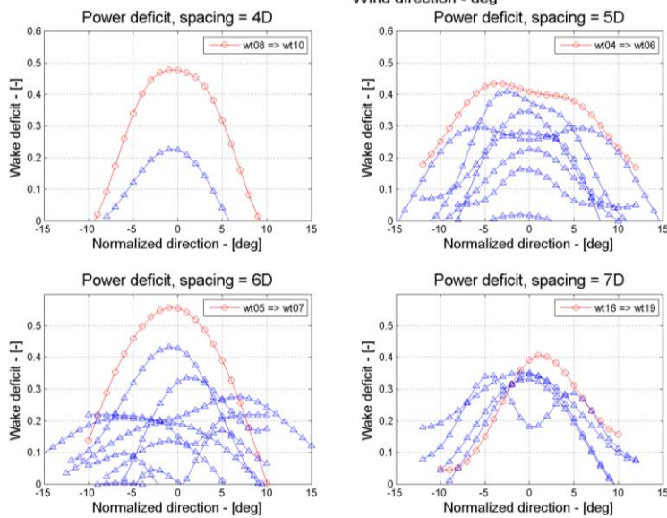
Figure 13: Power deficit (fitted) distributions between pairs of turbines with 4, 5, 6 or 7D spacing.
