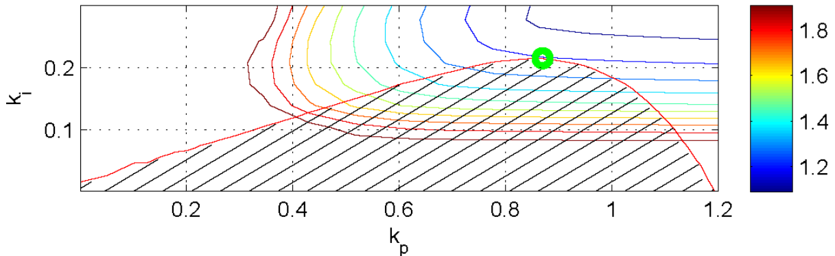
Figure 5: Contour plot of IAE overlaid with the hatched area showing M_t \leq 1.25
