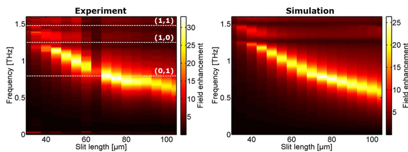
Figure 2. Experimental (left) and simulation (right) results of field enhancement inside slits when the length ( L ) is varied and the lattice parameters are P_x = 70 \mu\text{m} and P_y = 110 \mu\text{m} . The white dashed lines indicate lattice modes.
