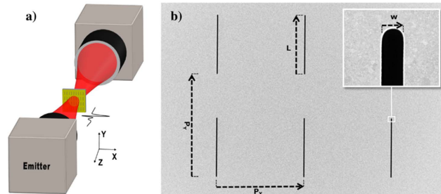
Figure 1. (a) Experimental configuration of a slit array measured with a THz-TDS system. (b) SEM image of a typical slit array. Then inset shows a zoom of a slit. In this specific case, L = 50 \mu\text{m} , P_x = 70 \mu\text{m} , P_y = 110 \mu\text{m} , and w = 1.5 \mu\text{m} .
