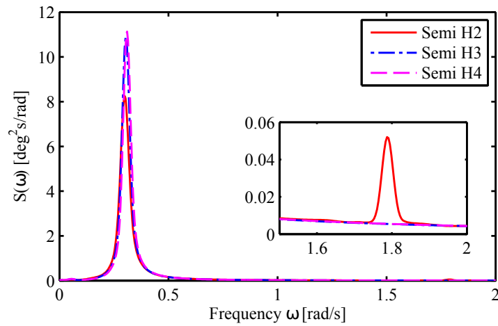
Figure 5. Power spectral analysis of pitch decay of the three floating VAWTs under steady wind with U_w=18 m/s.
