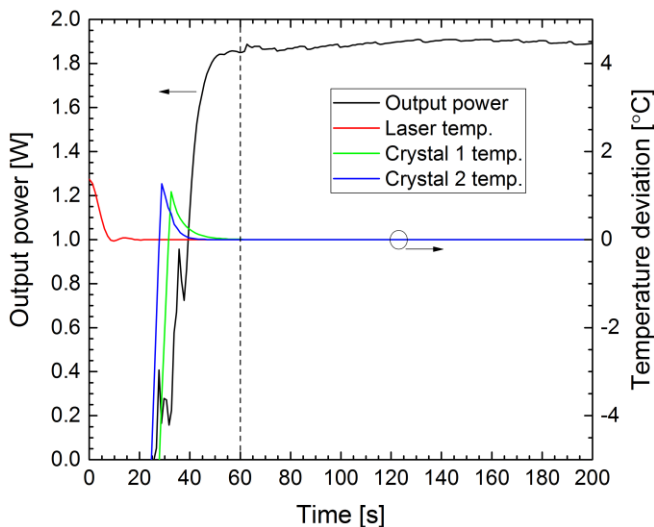
Fig. 4. Measurement of the laser system parameters during a start-up procedure. Both measurements are performed with the laser diode operating at 20^\circ\text{C} , 350 mA ridge current and 10.5 A tapered current.
