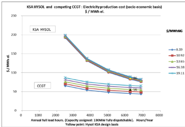
Fig. 4 Electricity production costs for Combined Cycle Gas Turbine (CCGT) and KSA HYSOL configuration, as function of load factor and NG price. Assumed: CO 2 costs = 40 $/tonCO 2 , R=4 %p.a., Lifetime=25 years. Unit: $/MWh el.
