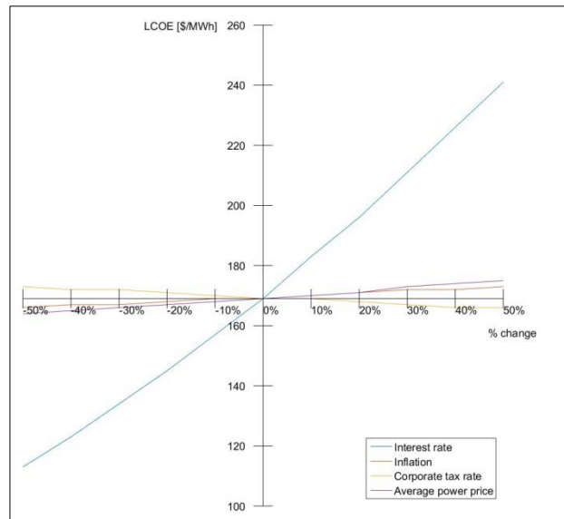
Fig. 8 Sensitivity analysis Private economic: economic parameters
