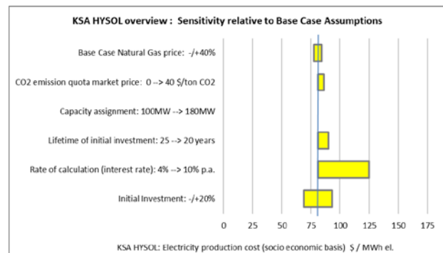
Fig. 5 KSA HYSOL results in overview: Electricity production costs (LCOE) - Sensitivity relative to Base Case Assumptions. Units: $/MWh el
