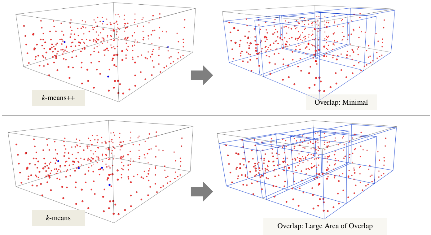
Figure 2. Comparison of initial cluster center by k -means and k -means++.
